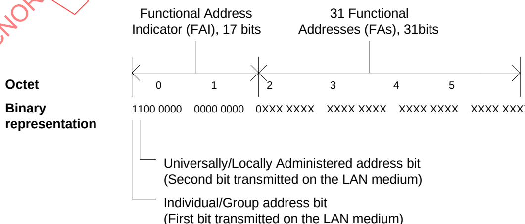
Figure 2 — Representation of Token Ring LAN Functional Addresses
