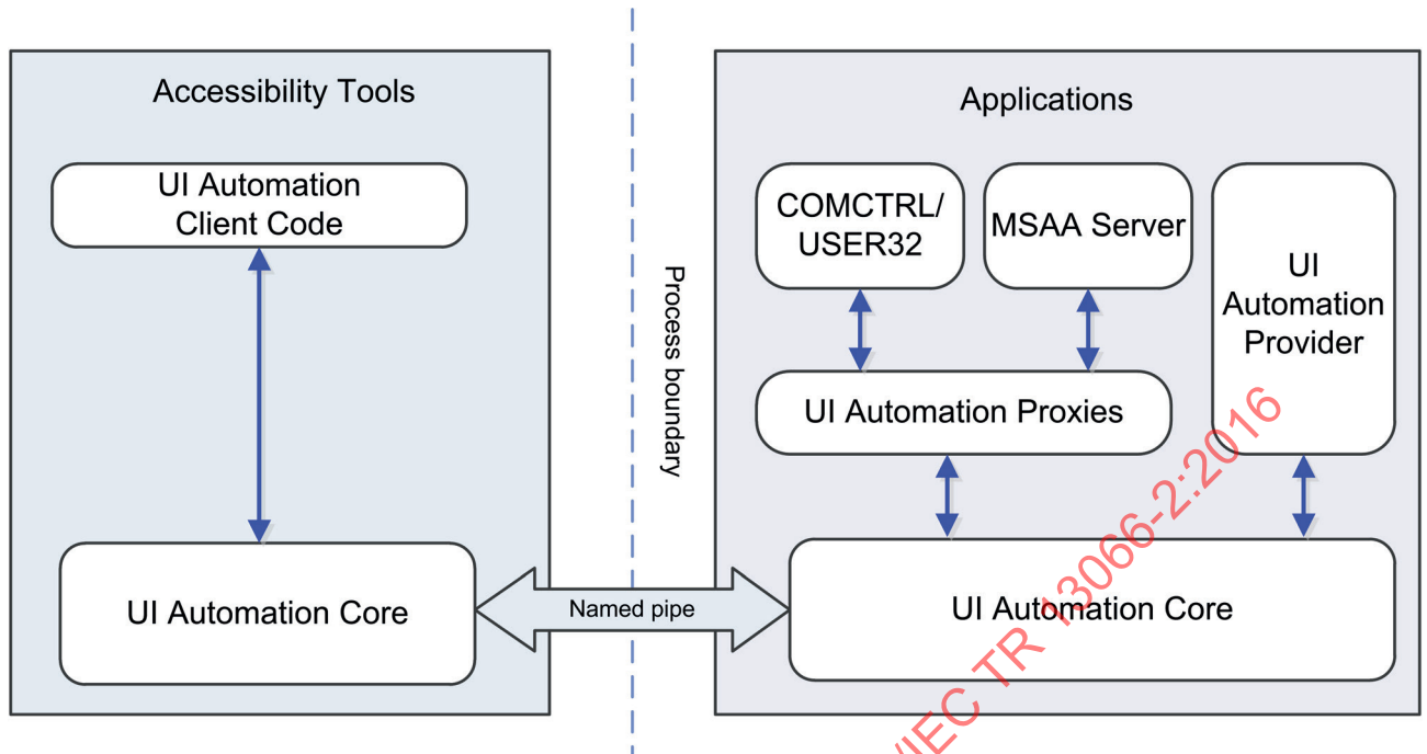
Figure 2 — UI Automation
