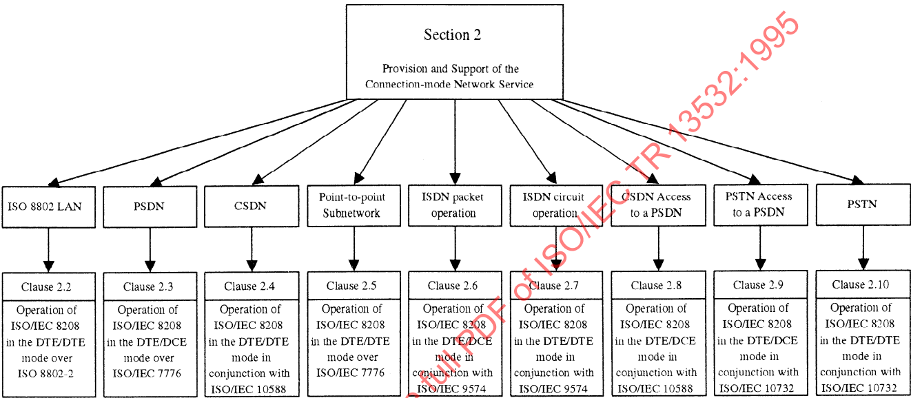
Figure 1 — Protocols to provide and support the connection-mode Network Service
