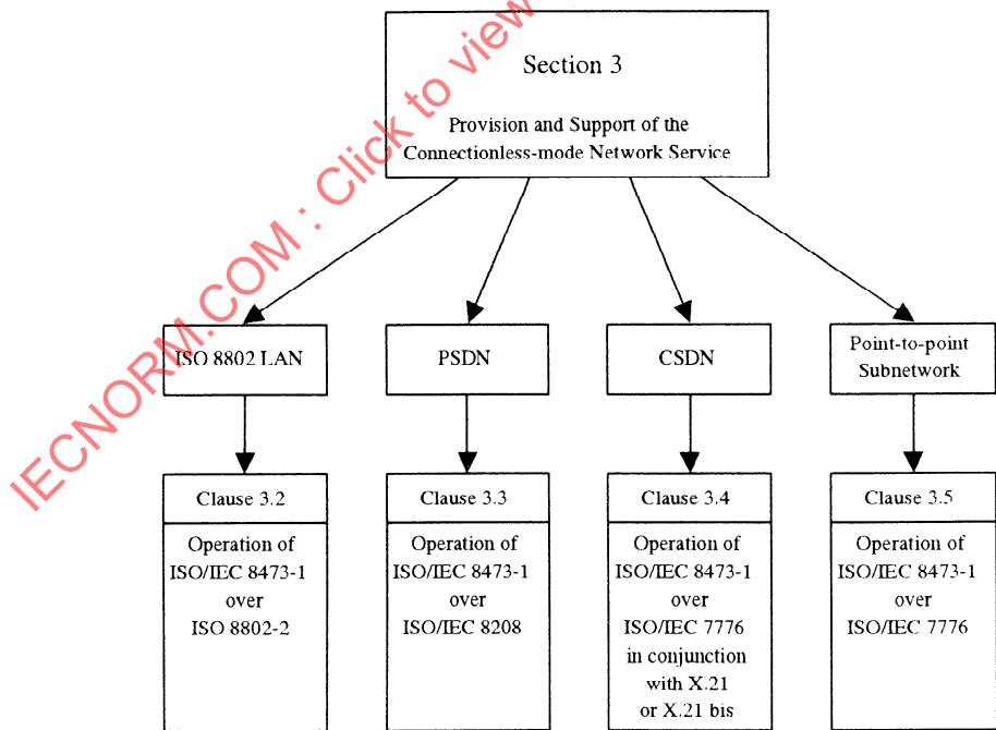
Figure 2 — Protocols to provide and support the connectionless-mode Network Service
