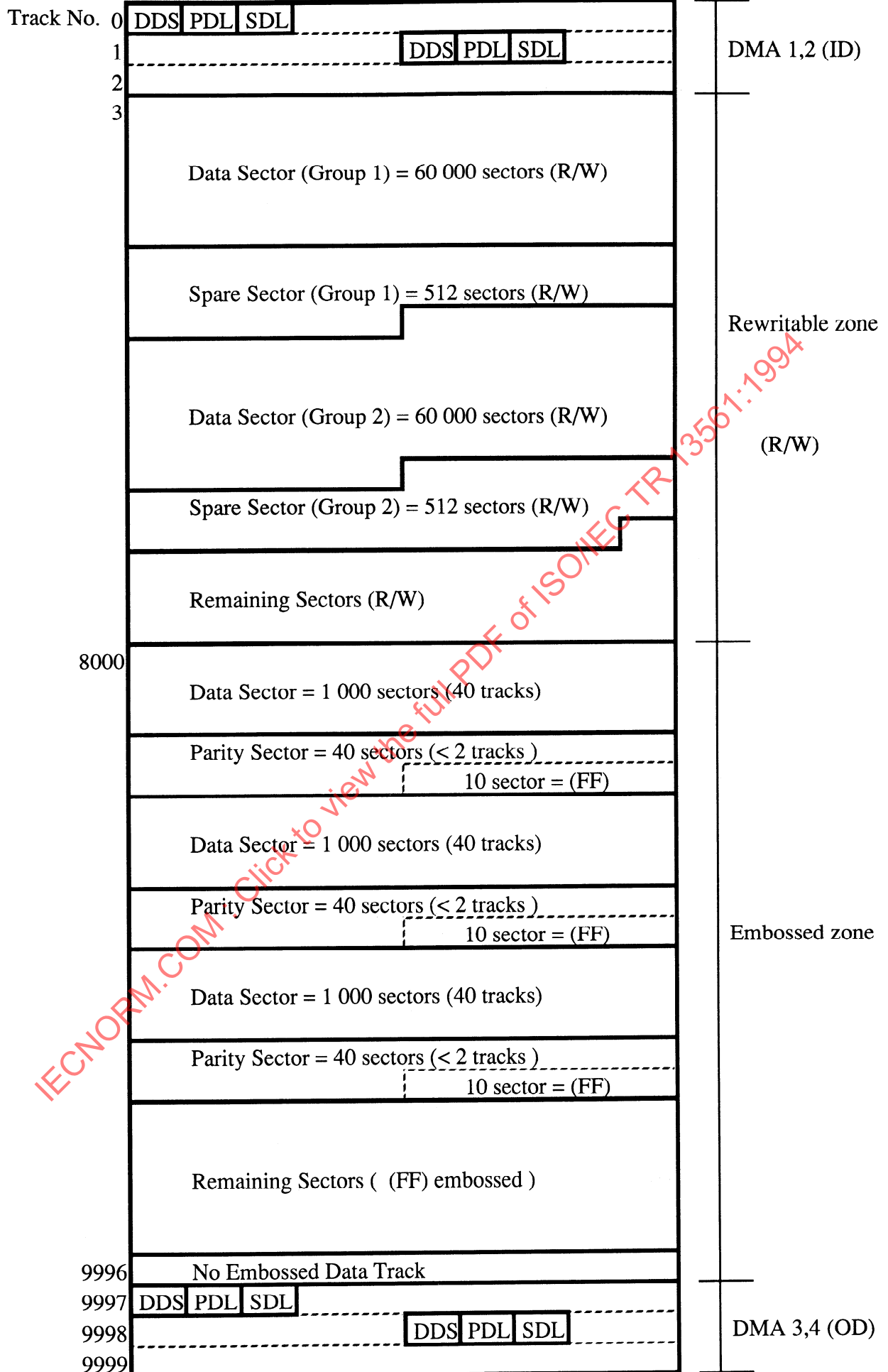
Figure 4 - Disk layout in case 1 (see.8)
