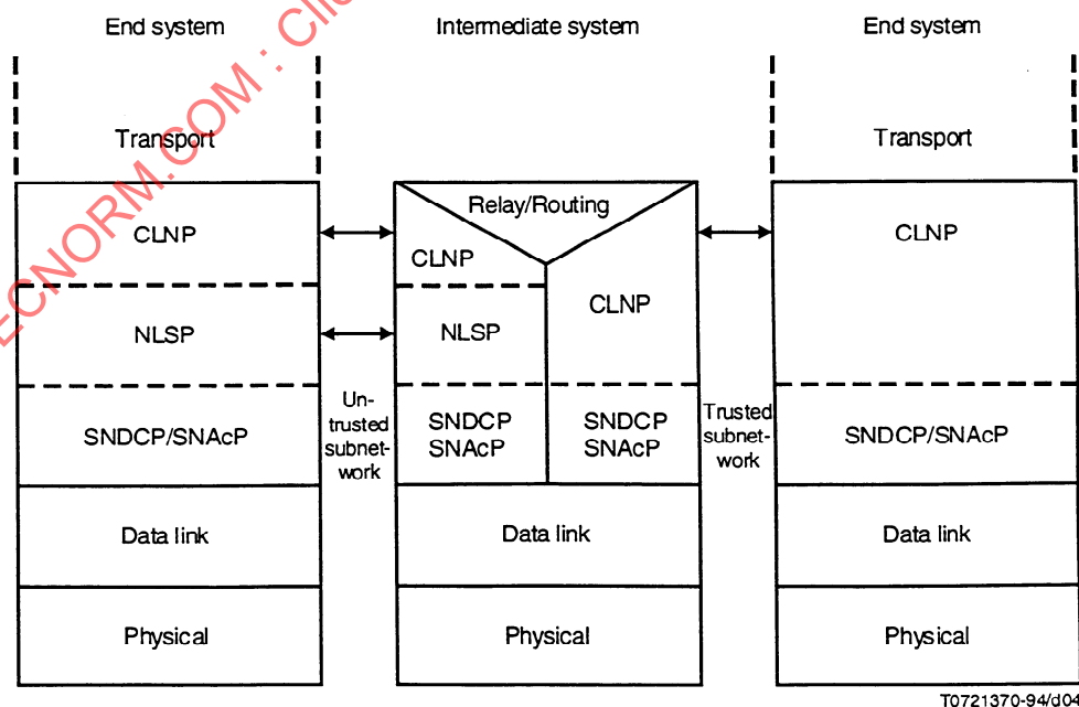
Figure 5 – Illustration of NLSP-CL with untrusted subnetwork
