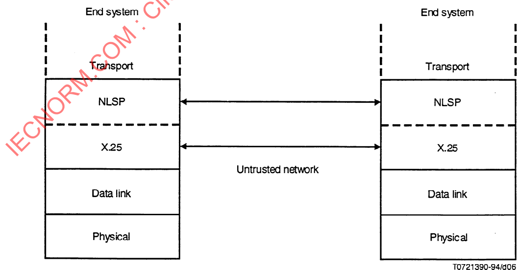
Figure 7 – Illustration of NLSP-CO between end systems
