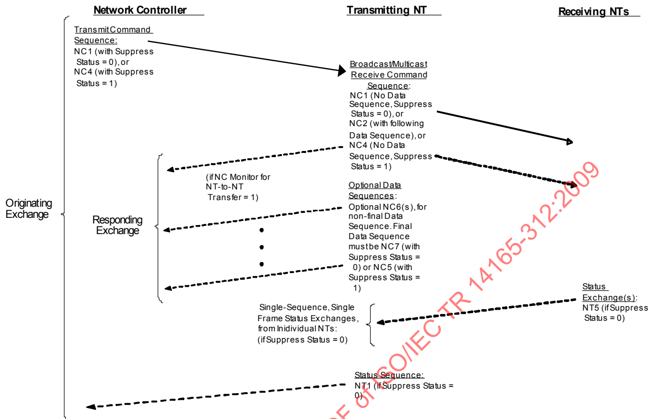
Figure 14 – Network Terminal to Multiple Network Terminals
