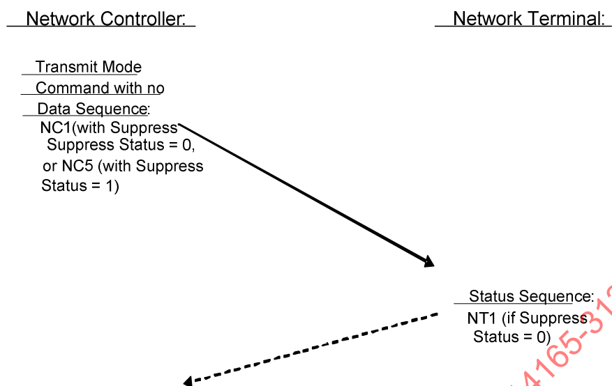
Figure 10 – Mode command without Data Word
