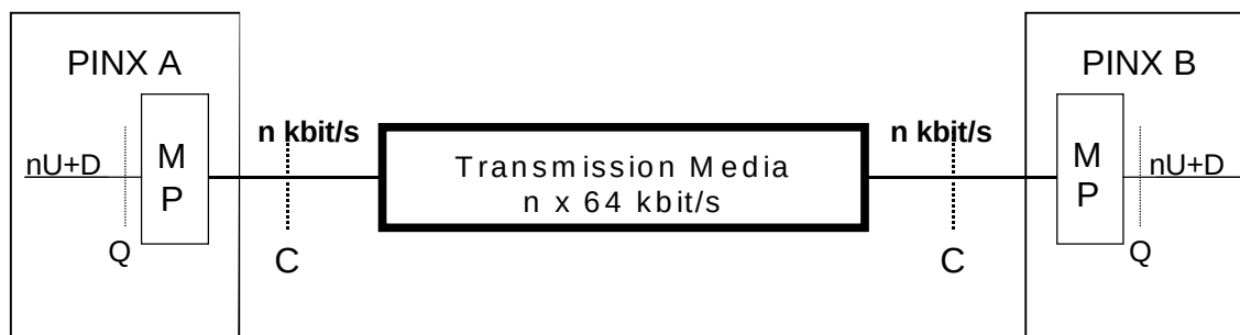
Figure 7 - Unstructured Transmission Link
