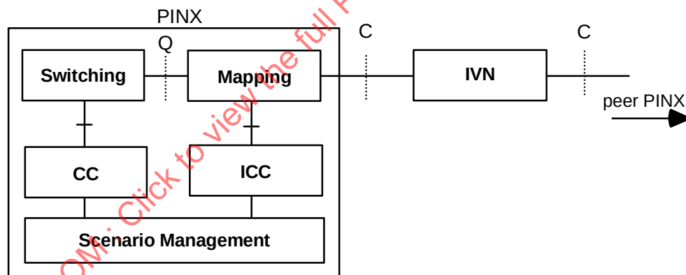
Figure 1 - PINX Reference Configuration (Excerpt)
