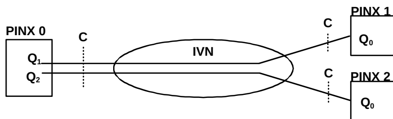
Figure 5 - Example of a PISN with Multiple IPLs
