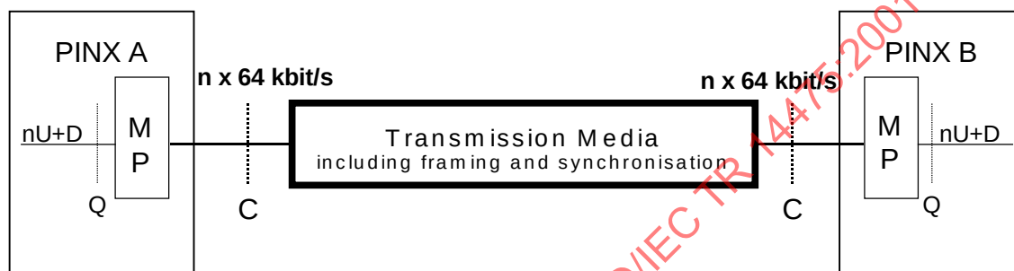
Figure 8 - Dedicated transmission System
