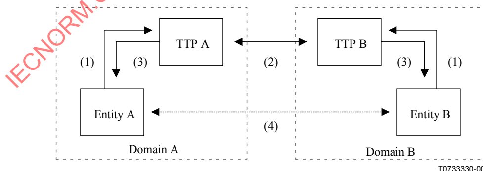
Figure 4 – Interworking of TTPs in Different Domains
