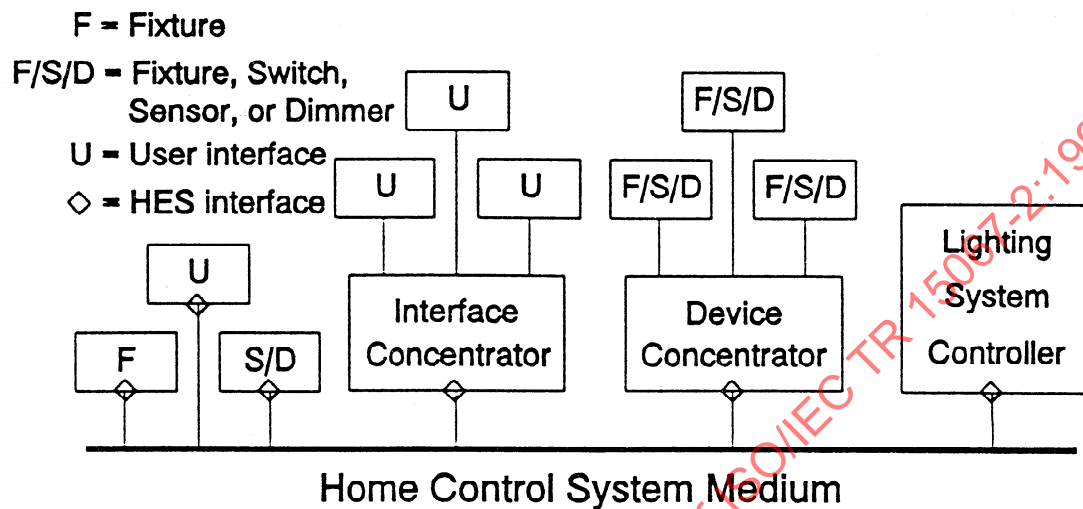
Figure 1: Example Illustrating Physical Components of an HES Lighting System
