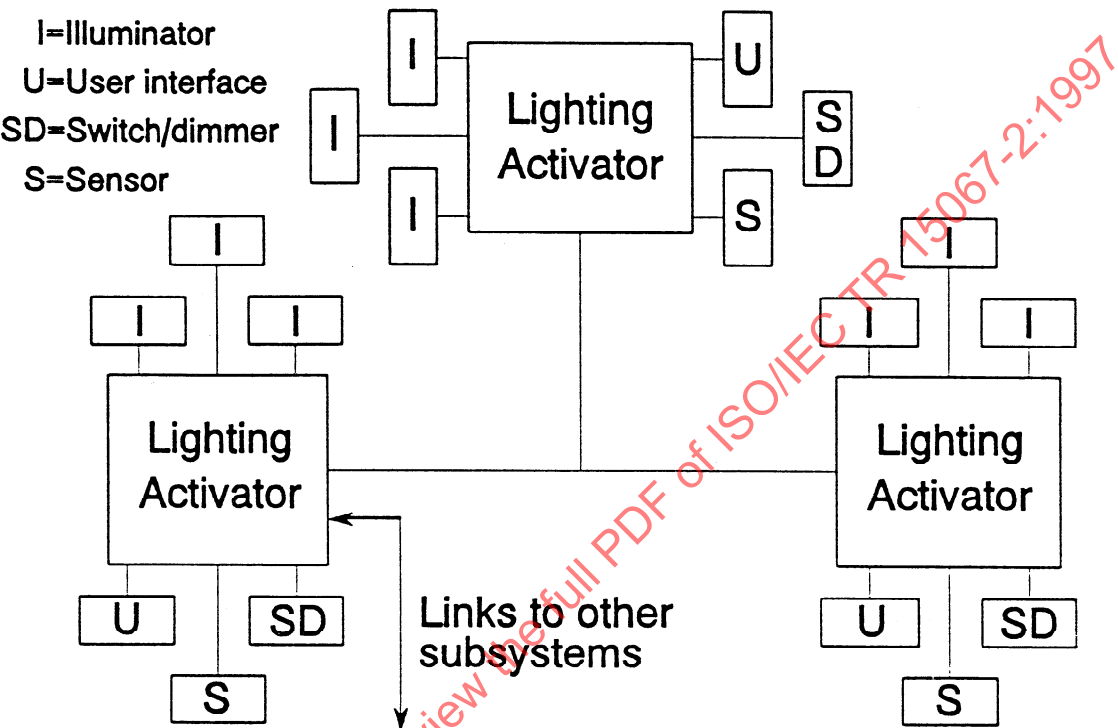
Figure 5: Logical Model of HES Distributed Lighting Control
