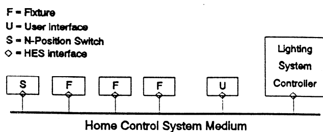
Figure 12: Case 4 — Physical Model
