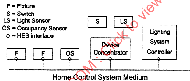
Figure 10: Case 3 — Physical Model
