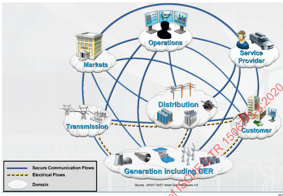
Figure 11 – NIST Smart Grid Conceptual Model
