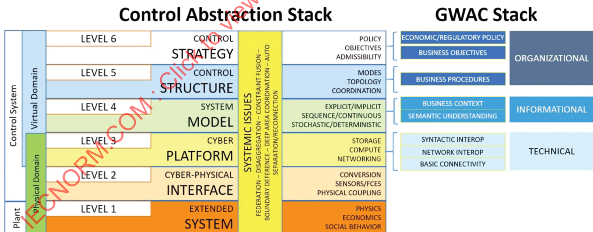
Figure 13 – Integrated Control Abstraction Stack/GWAC Stack model
