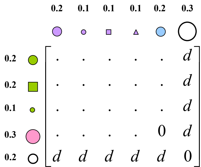
Figure AMD2-4 — Binary-distance matrix from the example in Figure AMD2-3
