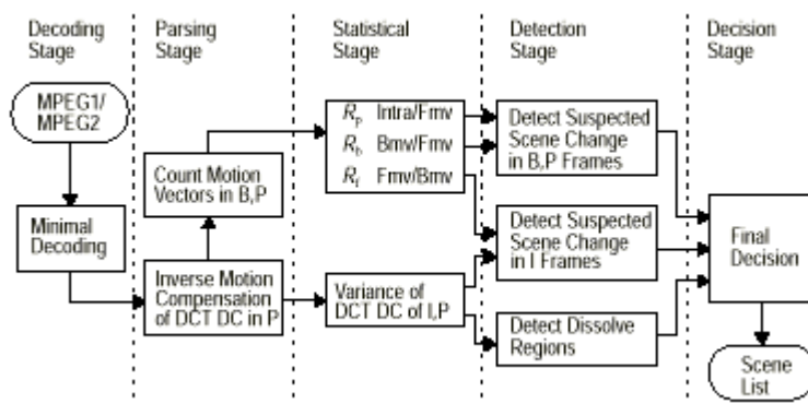
Figure 25 - The Block diagram of the scene change detection algorithm.
