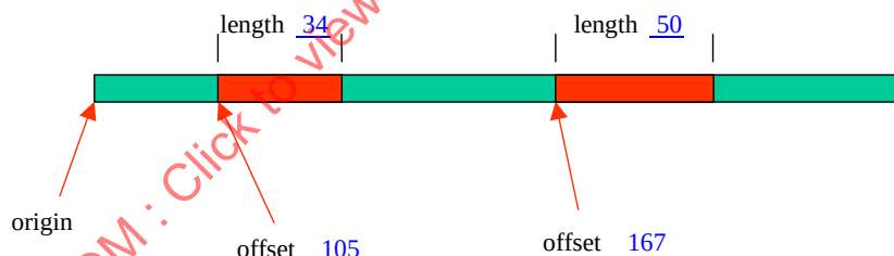
Figure 13 - Example of a media space mask.
