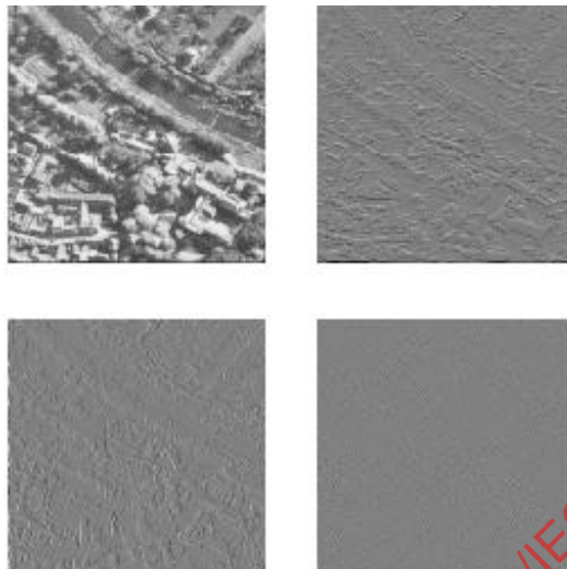
Figure 59 - Example View Set with a set of Frequency Views that are image subbands. This View Set is complete and nonredundant.
