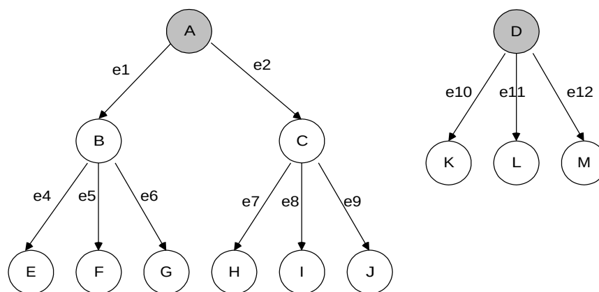
Figure 45 - An example of the key-frame selection algorithm based on fidelity values.
