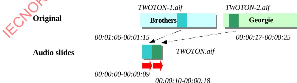
Figure 53 - Example of an audio summary with multiple sources.
