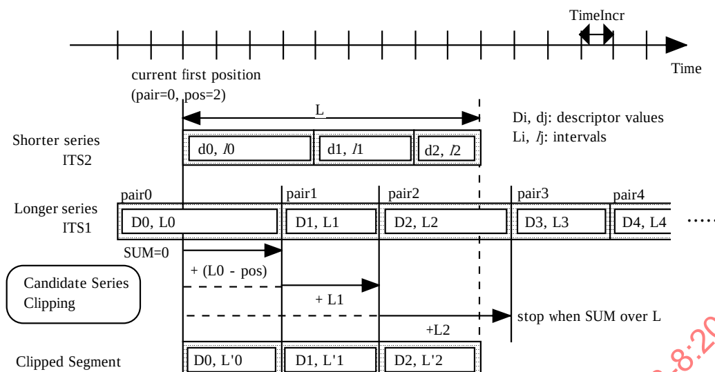
Figure 69 - Overview of video segment clipping.
