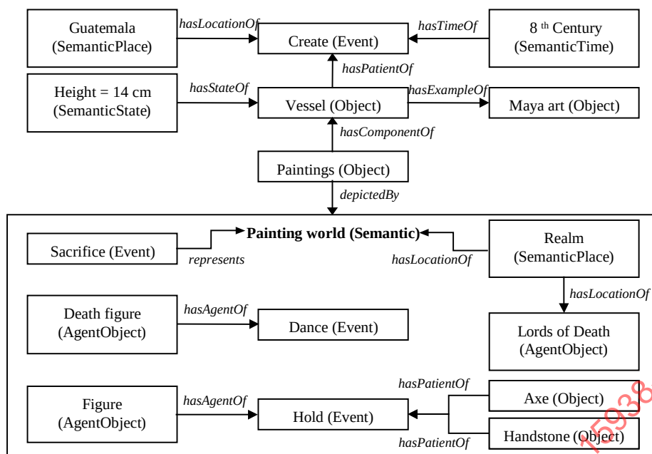
Figure 41 - Example semantic description of a Mayan vessel.
