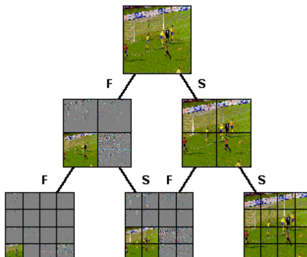
Figure 60 - shows an example Space and Frequency Graph decomposition of an image. The Space and Frequency Graph structure includes node elements that correspond to the different space and frequency views of the image, which consist of views in space (spatial segments), frequency (wavelet subbands), and space and frequency (wavelet subbands of spatial segments). The Space and Frequency Graph structure includes also transition elements that indicate the analysis and synthesis dependencies among the views. For example, in the figure, the "S" transitions indicate spatial decomposition while the "F" transitions indicate frequency or subband decomposition.
