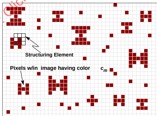
Figure 84 - Un-structured iso-color plane
