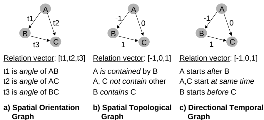
Figure 36 - Examples of spatio-temporal relation graphs.
