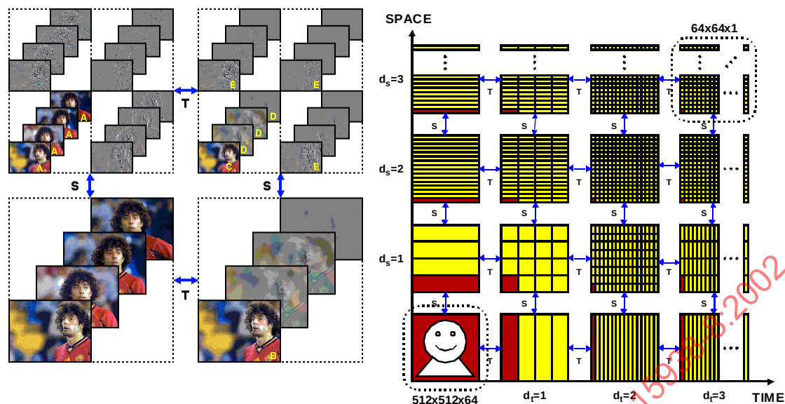
Figure 61 - Example of Video View Graph. (a) Basic spatial- and temporal-frequency decomposition building block, (b) Example video view graph of depth three in spatial- and temporal-frequency.
