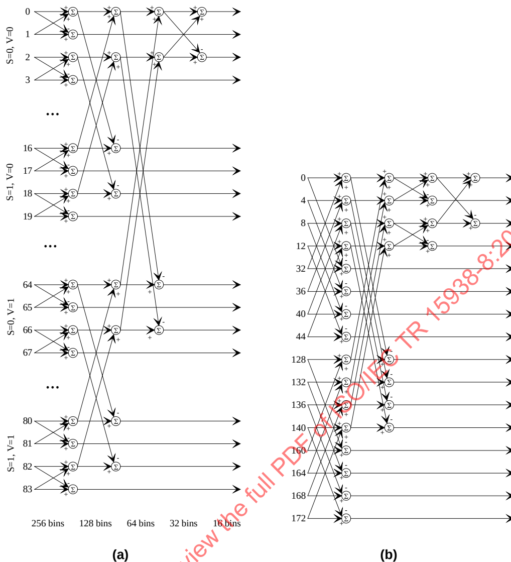
Figure 81 - Haar transform of 256-bin HSV color histogram. (a) first four levels, (b) levels 5-8 (index values corresponding to the indices of bins in a HSV color histogram with 256 bins, according to Table 11 of normative part an index assignment of uniform color quantization D)
