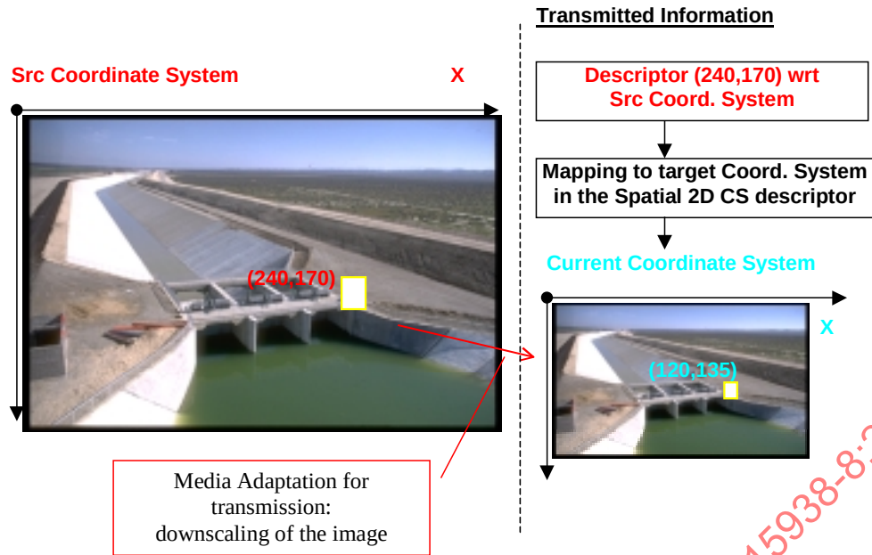
Figure 77 - Coordinate changes by scaling of an image: original descriptor in the src coordinate system and its mapping into the target coordinate system (in this example both pixel based).
