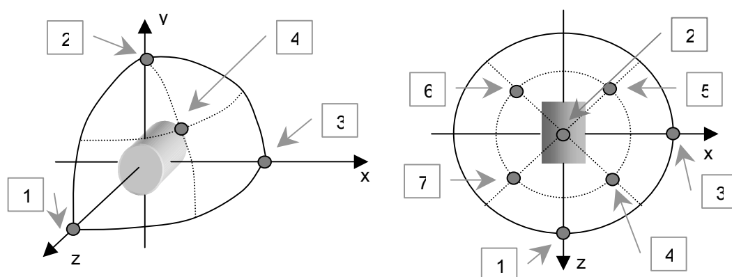
Figure 72 - Viewing directions onto the 3D object in the origin: Left: perspective view and view directions in the first octant, Right: top view and view directions in the hemisphere y > 0 .
