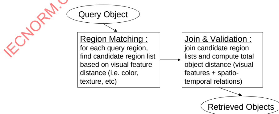
Figure 31 - The video object query model.
