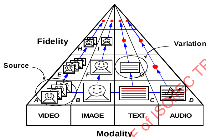
Figure 62 - Illustration of different variations of a source content. The eight variation contents have different modalities (video, image, text, audio) and fidelities with respect to the source content.
