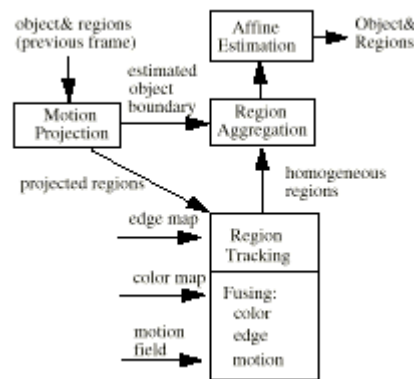
Figure 30 - Automatic semantic object tracking.
