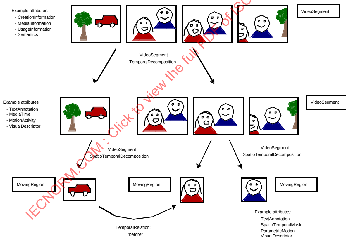
Figure 12 - Illustration of the description of a video segment using tools for describing the structure of multimedia content.
