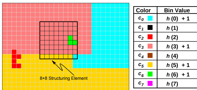
Figure 85 - Accumulation of Color Structure Histogram.
