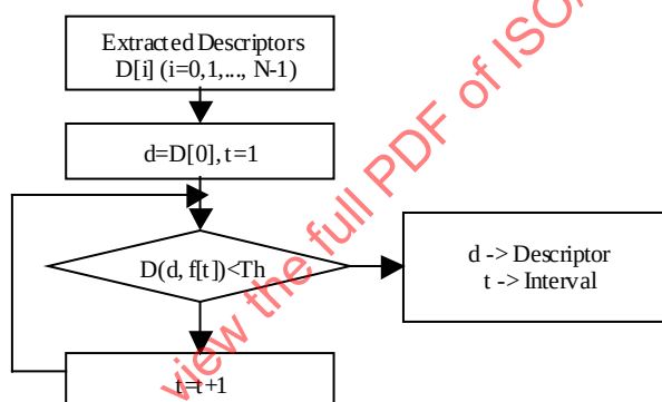
Figure 68 - Flow chart to extract time intervals.
