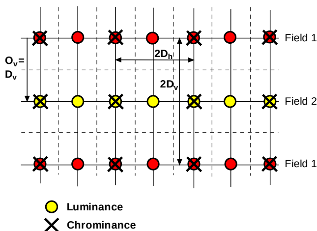
Figure 10 - Illustration of the siting of luminance and chrominance samples for 4:2:2 data (i.e., MPEG-2 interlaced color sampling YCbCr 4:2:2).
