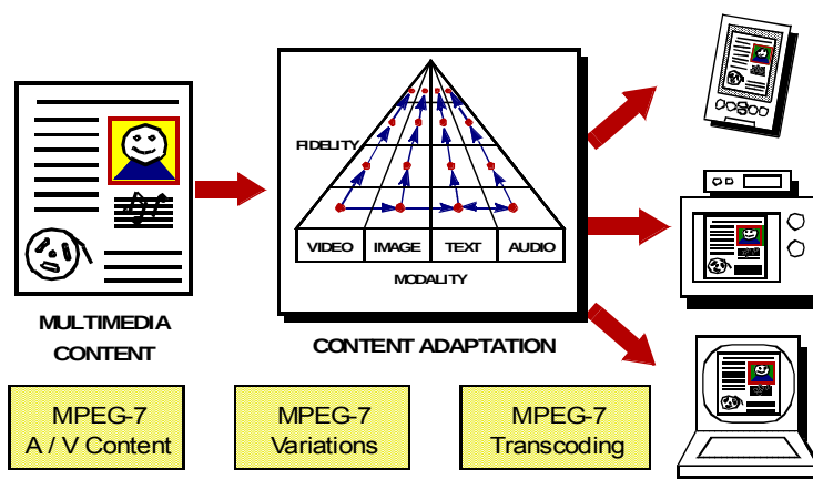
Figure 63 - Illustration of an example application of Universal Multimedia Access (UMA) in which the appropriate variations of the multimedia programs are selected according to the capabilities of the terminal devices. The MPEG-7 transcoding hints may be used in addition to further adapt the programs to the devices.
