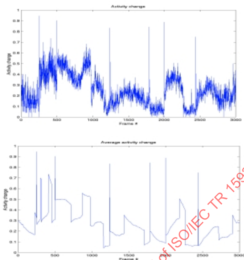
Figure 49 - Activity change (top). Segmented signal (bottom).
