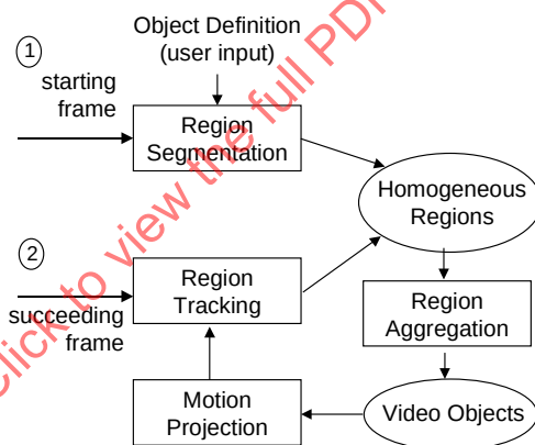
Figure 28 - General Structure of AMOS.
