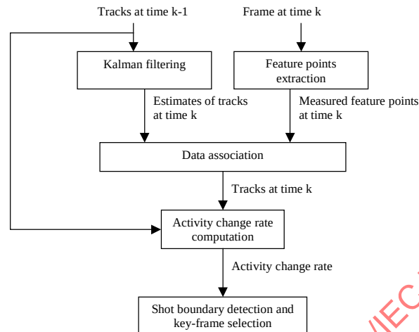
Figure 47 - Shot boundary detection and key-frame selection.
