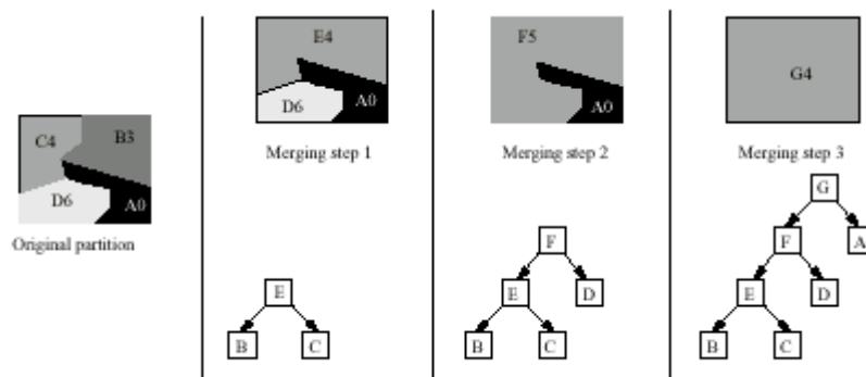
Figure 19 - Example of Binary Partition Tree creation with a region merging algorithm.
