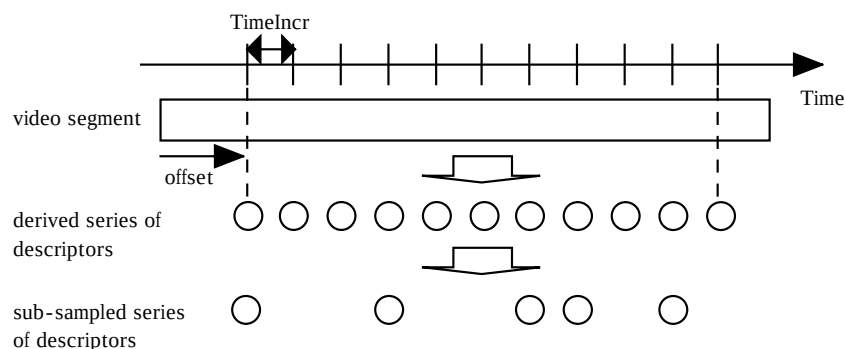
Figure 67 - Extraction method of a series of descriptors.
