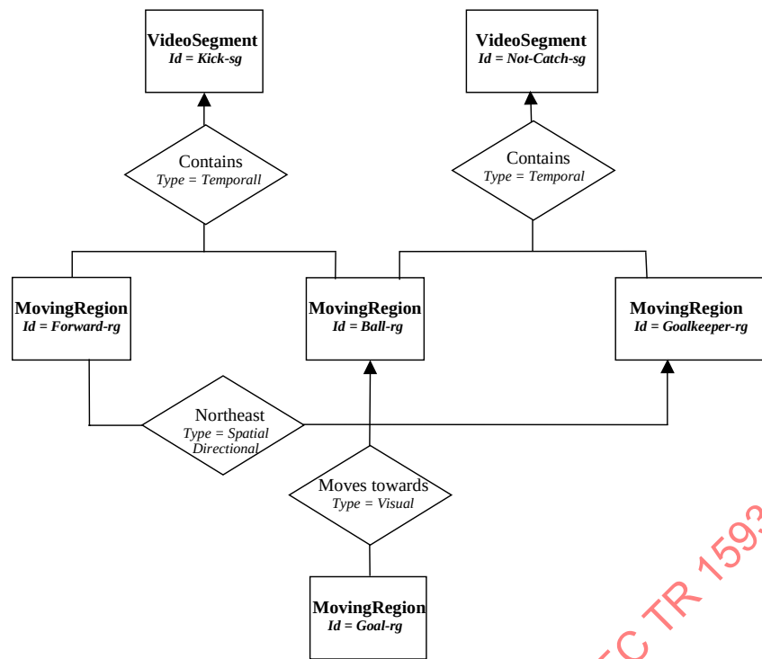
Figure 38 - Examples of relationships among video segments and moving regions.
