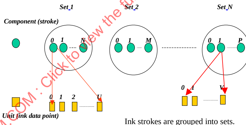
Figure 15 - Example of an ordered group mask.
