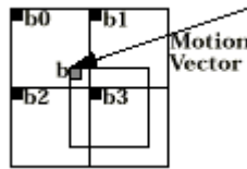
Figure 27 - Inverse Motion Compensation of DCT DC coefficient.
