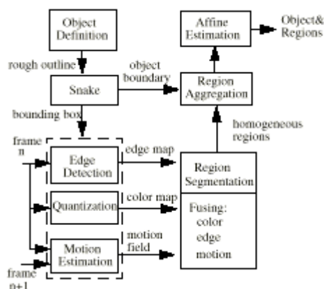
Figure 29 - Object segmentation at starting frame.
