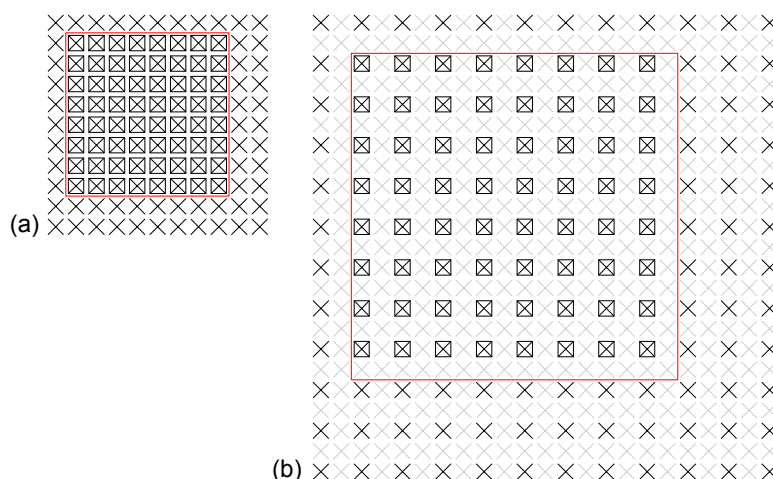
Figure 86 - (a): Structuring Element spatial extent and accumulation for K=1 (nominal operation). (b): For (K=2).
