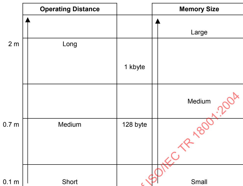
Figure 1 – Definition of Operation Distance and Memory Size
