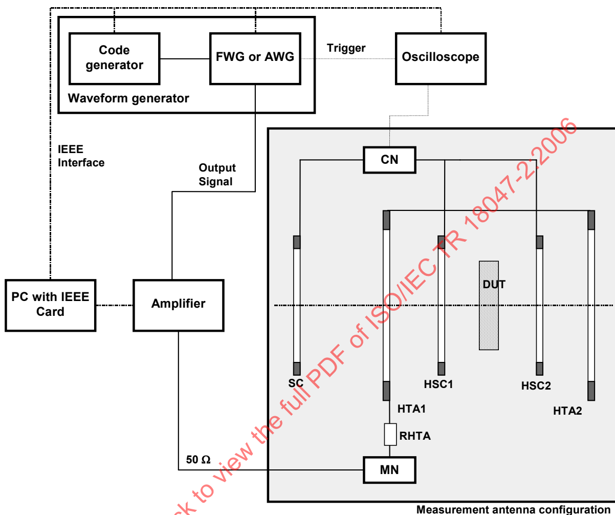
Figure 1 — Functional diagram
