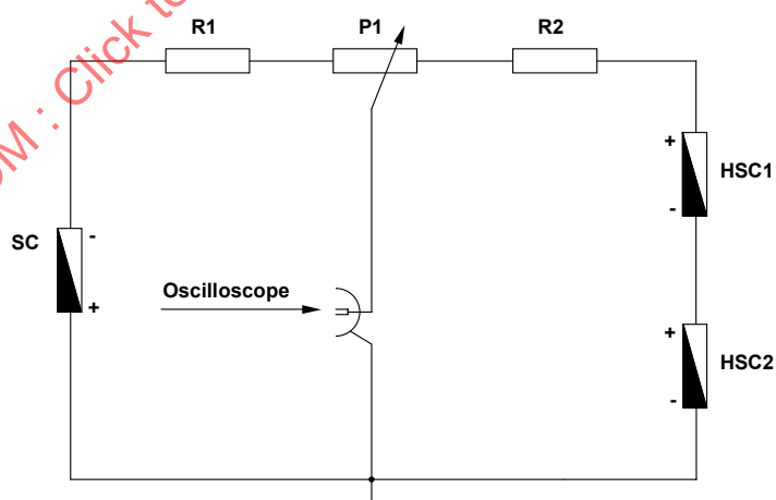
Figure 6 — Compensation network
