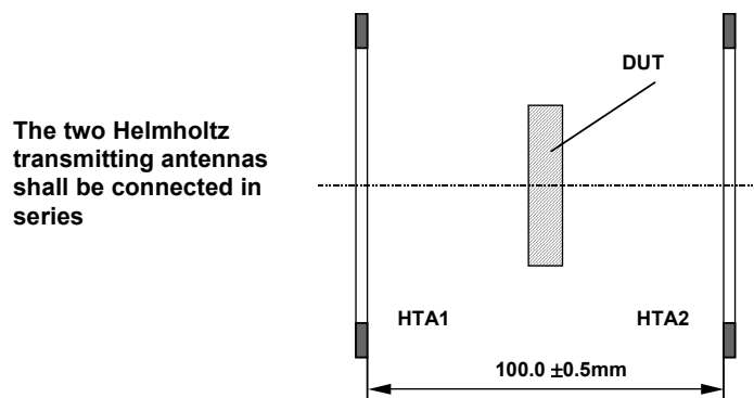
Figure 3 — Helmholtz setup
