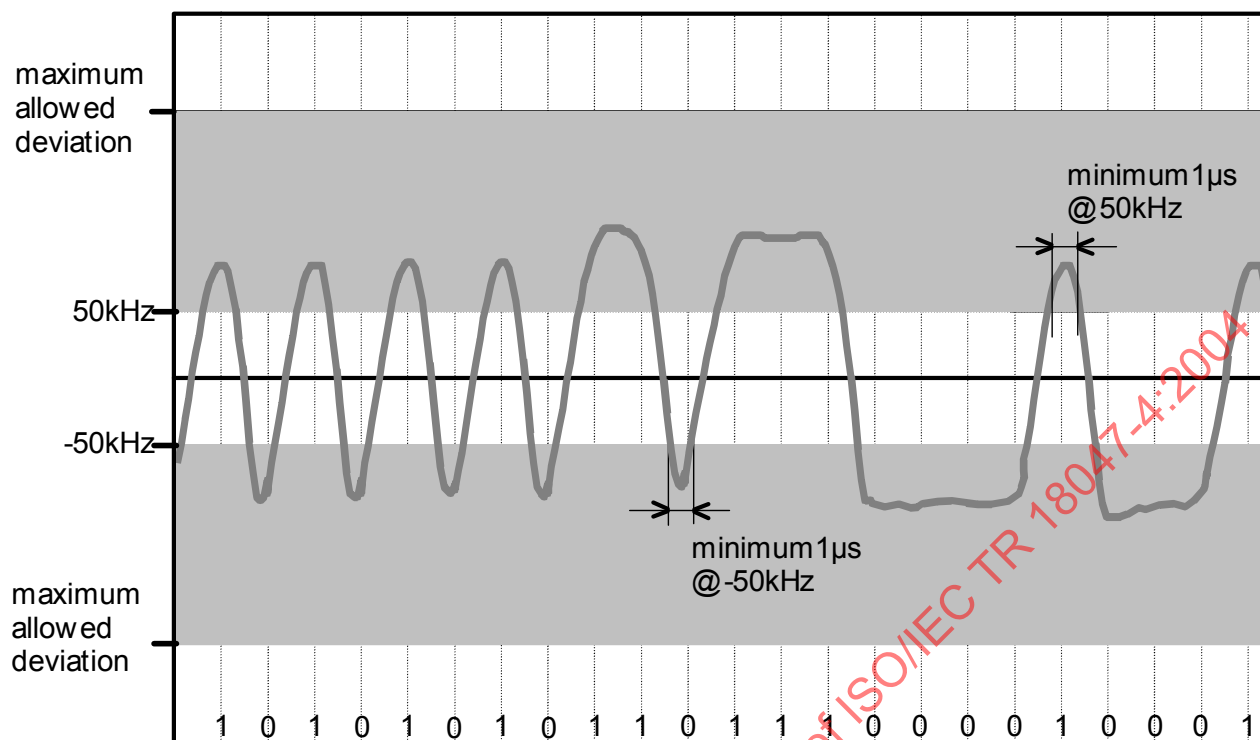
Figure 2 – Mask representation of the limits for modulation characteristic
