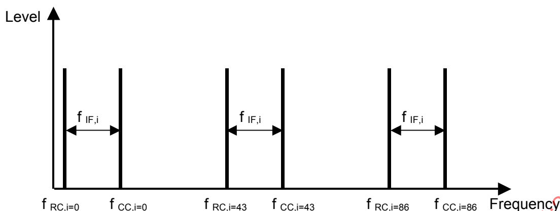
Figure 1 – Reference and communication carrier for 3 channel numbers i (0, 43, 86)
