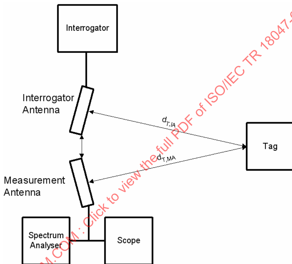
Figure 4 — Tag backscatter test setup
