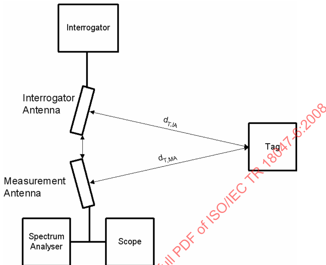
Figure 4 — Tag demodulation test setup
