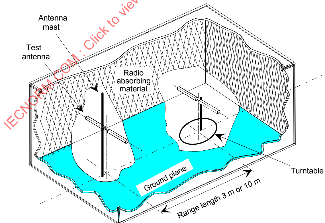
Figure A.2 — A typical anechoic chamber with a conductive ground plane
