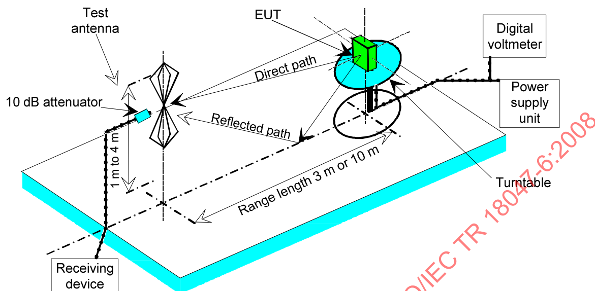
Figure A.4 — Measuring arrangement on ground plane test site (OATS set-up for spurious emission testing)
