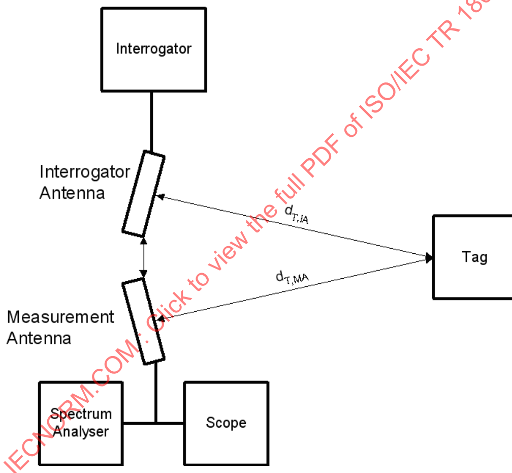
Figure 4 — Tag demodulation test setup
