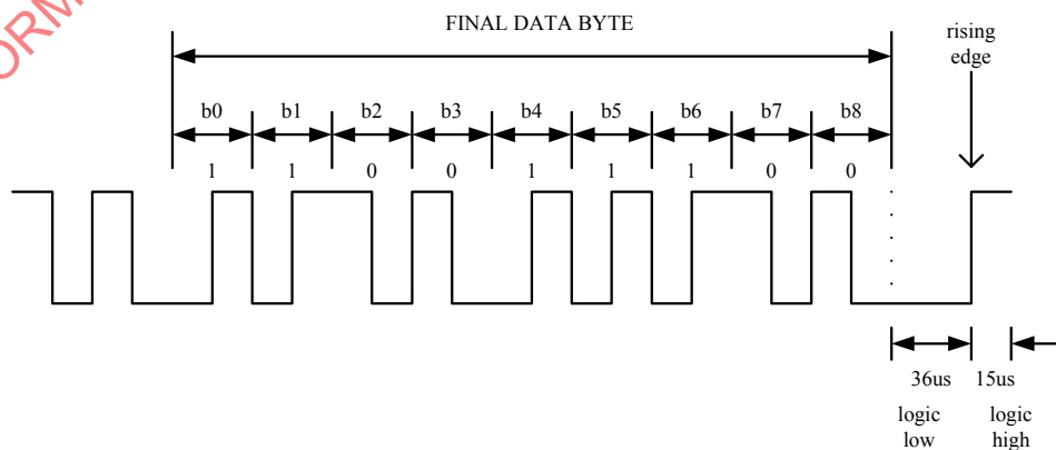
Figure 8 — Final Data Byte Timing
