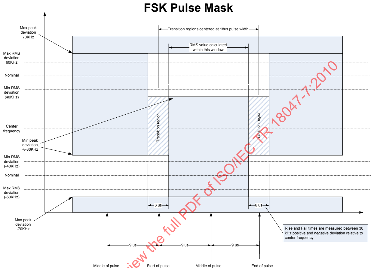
Figure 3 — FSK Pulse Mask
