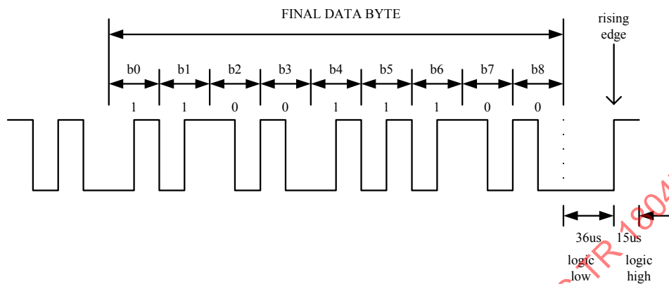
Figure 10 — Final Data Byte Timing
