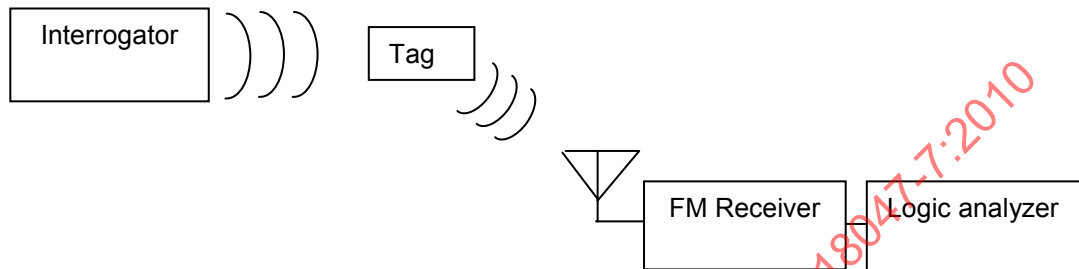
Figure 5 — Co-Header signal testing setup
