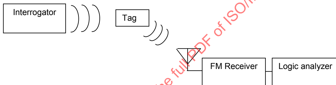
Figure 4 — Wakeup Header testing setup
