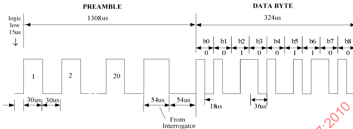
Figure 6 — Interrogator data communication and timing
