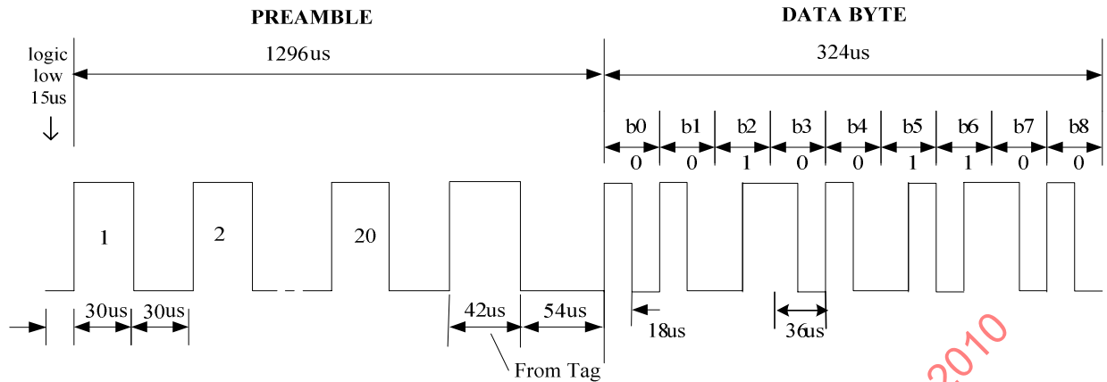
Figure 9 — Tag data communication and timing
