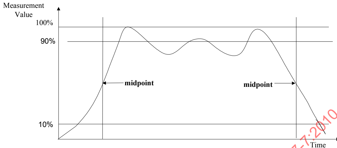
Figure 7 — Signal example with reference levels
