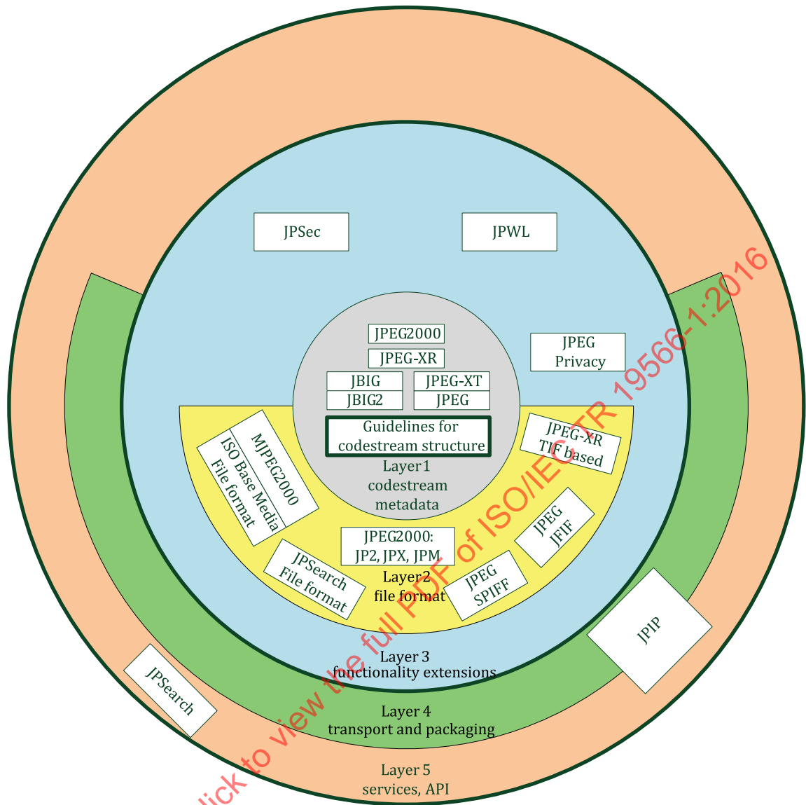
Figure 1 — Layered architecture of the JPEG Systems
