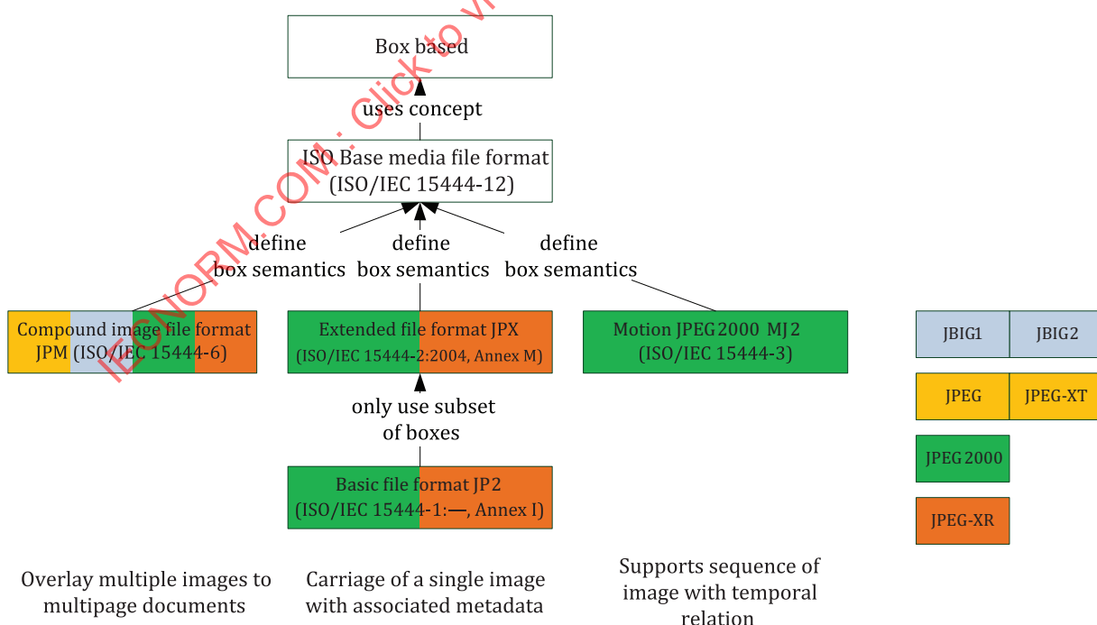
Figure C.1 — Box-based file formats in JPEG Standards
