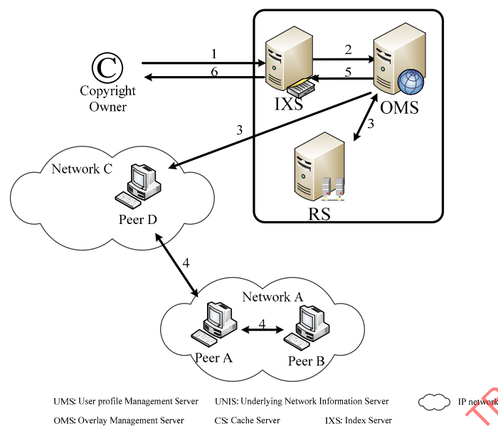
Figure 8 — Forced stop of illegal distribution
