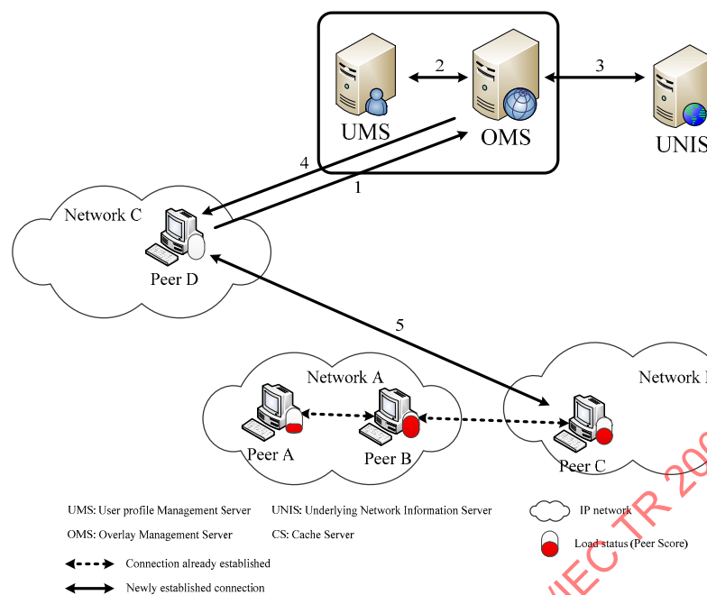
Figure 6 — Control flow for load balancing
