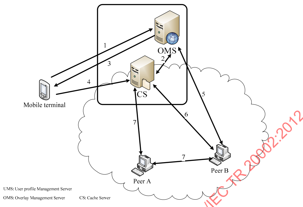
Figure 11 — Flows for resource delegation
