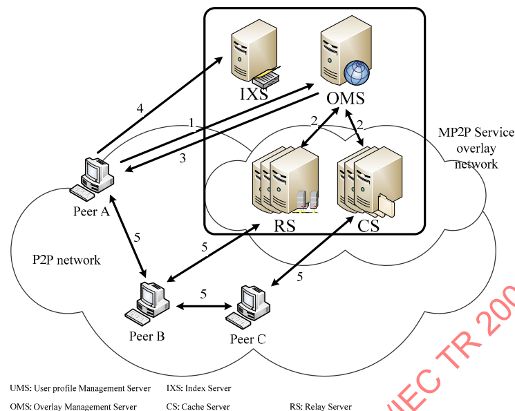
Figure 10 — Configuration of MP2P service overlay network
