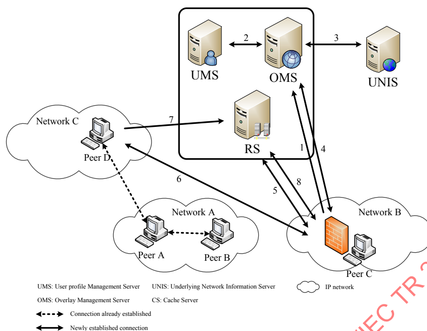
Figure 7 — NAT/Firewall traversal in MP2P network
