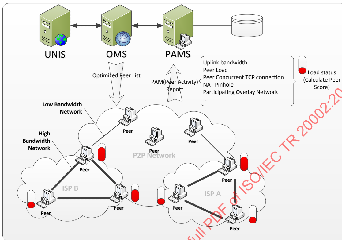
Figure A.2 — Use case of file distribution in MP2P
