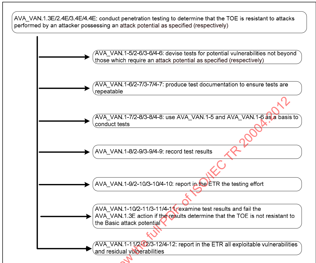
Figure 2 — “Penetration testing” evaluator action summary
