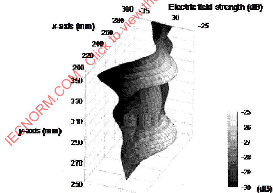
Figure A.14b —3D electric field distributions around the AIMD for 950 MHz
