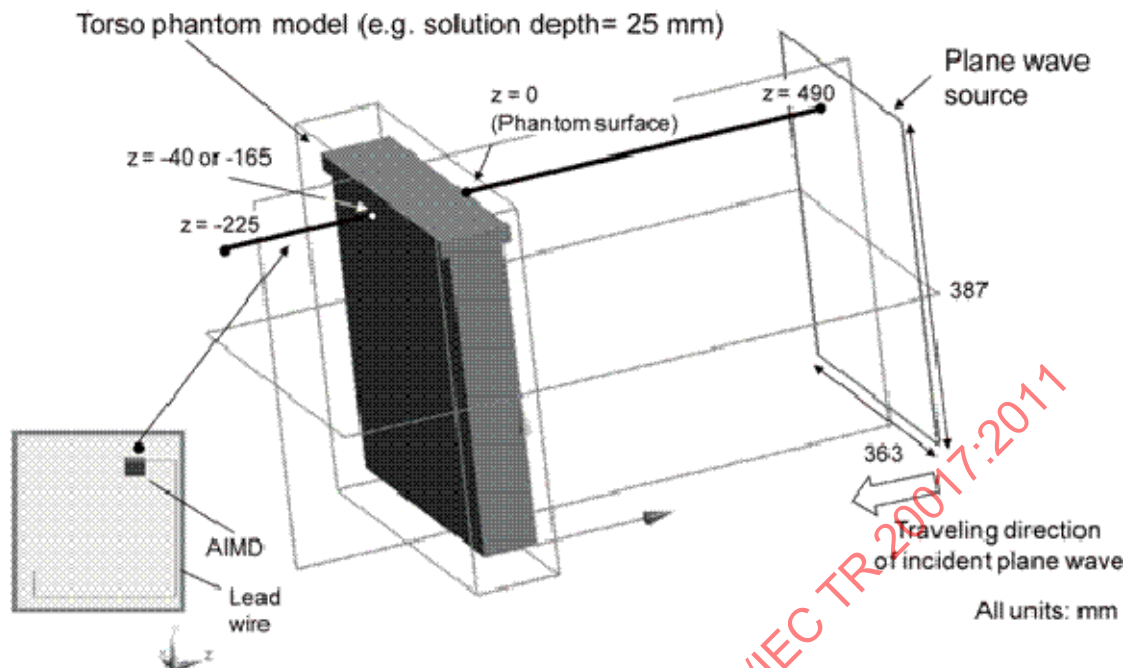
Figure A.9 — Analysis model for thickness simulations
