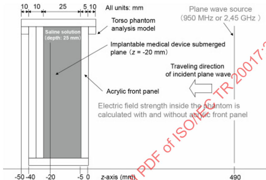
Figure A.6 — Analysis model for torso phantom
