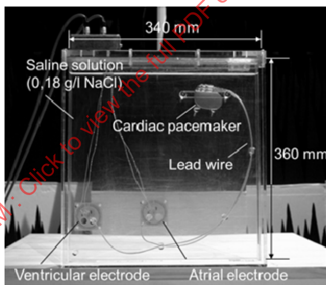
Figure A.5 — Vertical torso phantom
