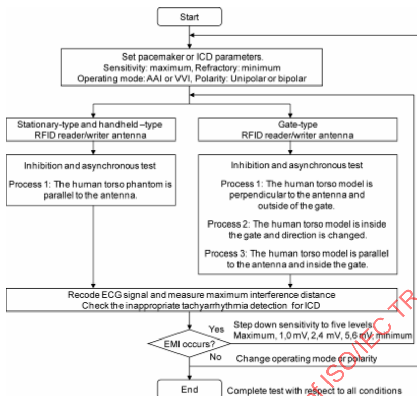
Figure A.17 — Fundamental measurement procedure
