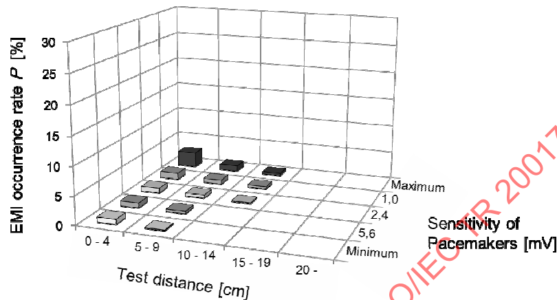
Figure A.26 — Test results of ISO/IEC 18000-3, Mode 1 stationary type RFID interrogators and pacemakers (Inhibition and asynchronous tests at different sensitivities)
