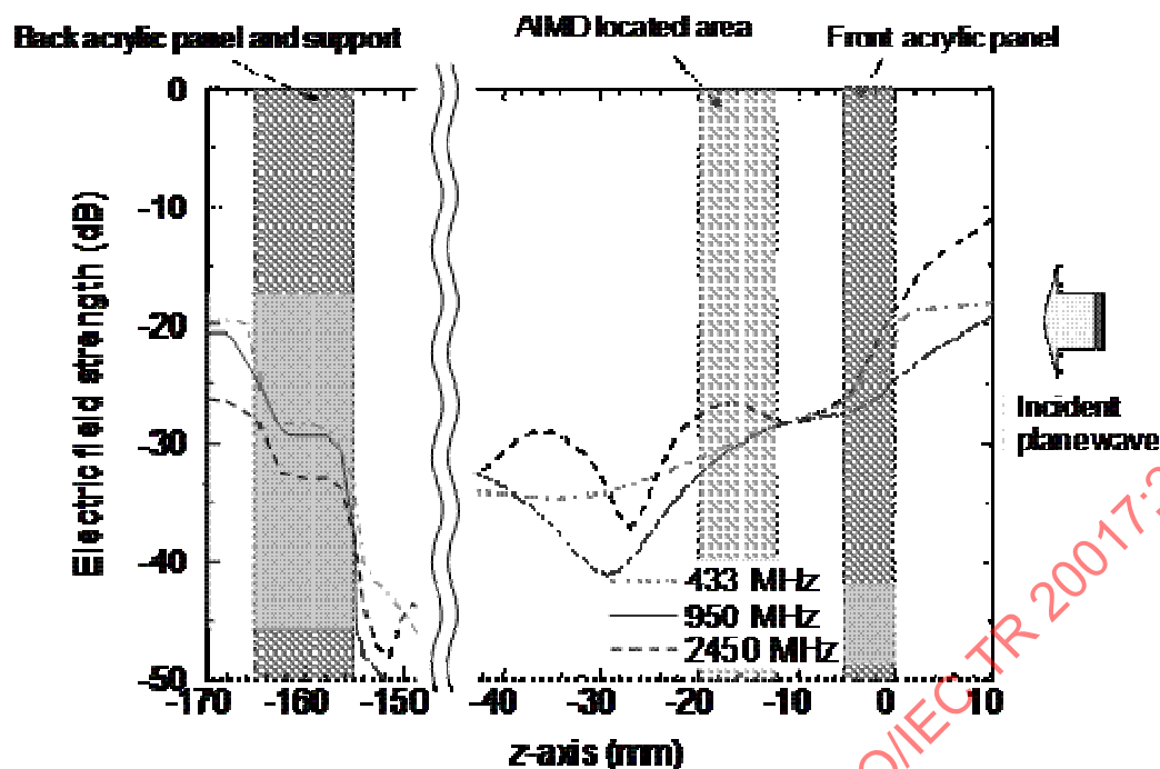
Figure A.11 — Electric fields for 150 mm thickness
