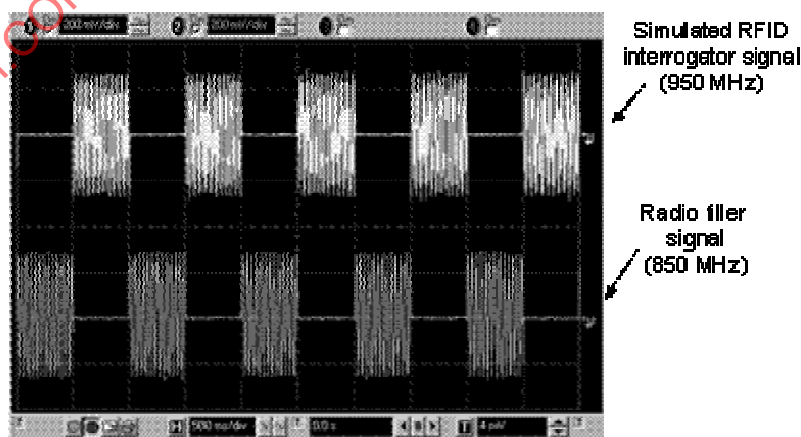
Figure A.45 — Waveforms of RFID interrogator and Radio filler signals
