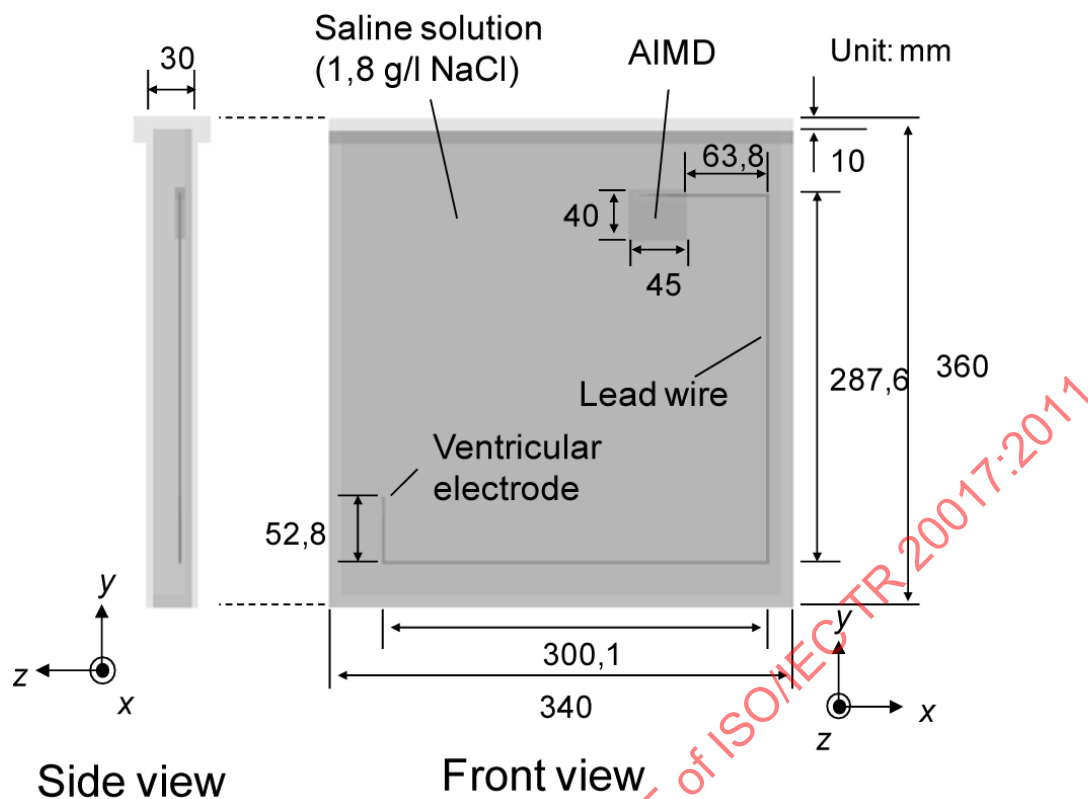
Figure A.35 — Numerical torso phantom with AIMD model
