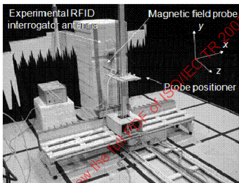
Figure A.37 — 3-D Measurement system for 13,56 MHz magnetic field distribution near antenna
