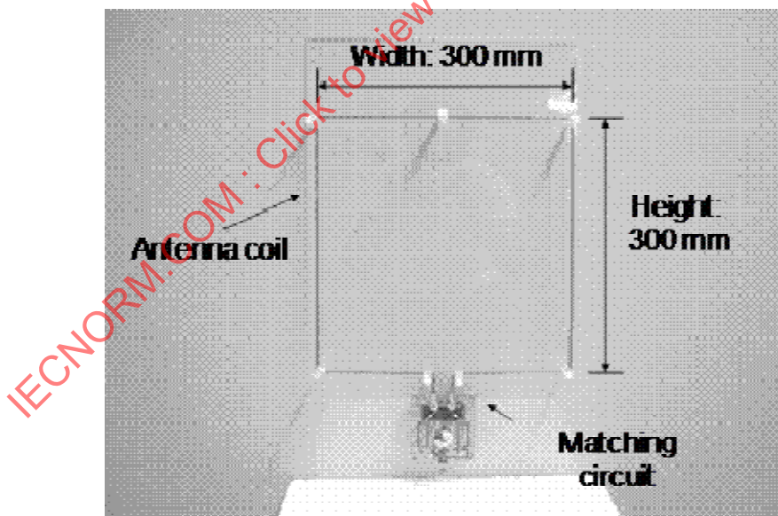
Figure A.36 — 13,56 MHz antenna model for experimental validation
