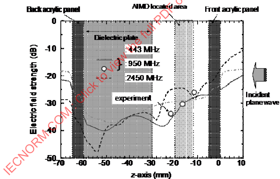
Figure A.13 — Standing waves inside the new phantom
