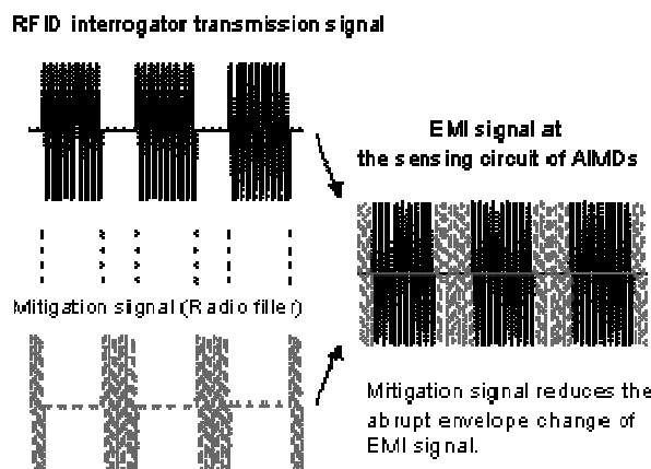
Figure A.42 — Fundamental structure of mitigation signal
