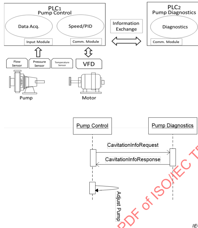
Figure 31 – Data Flow of Integrated Smart Pump System
