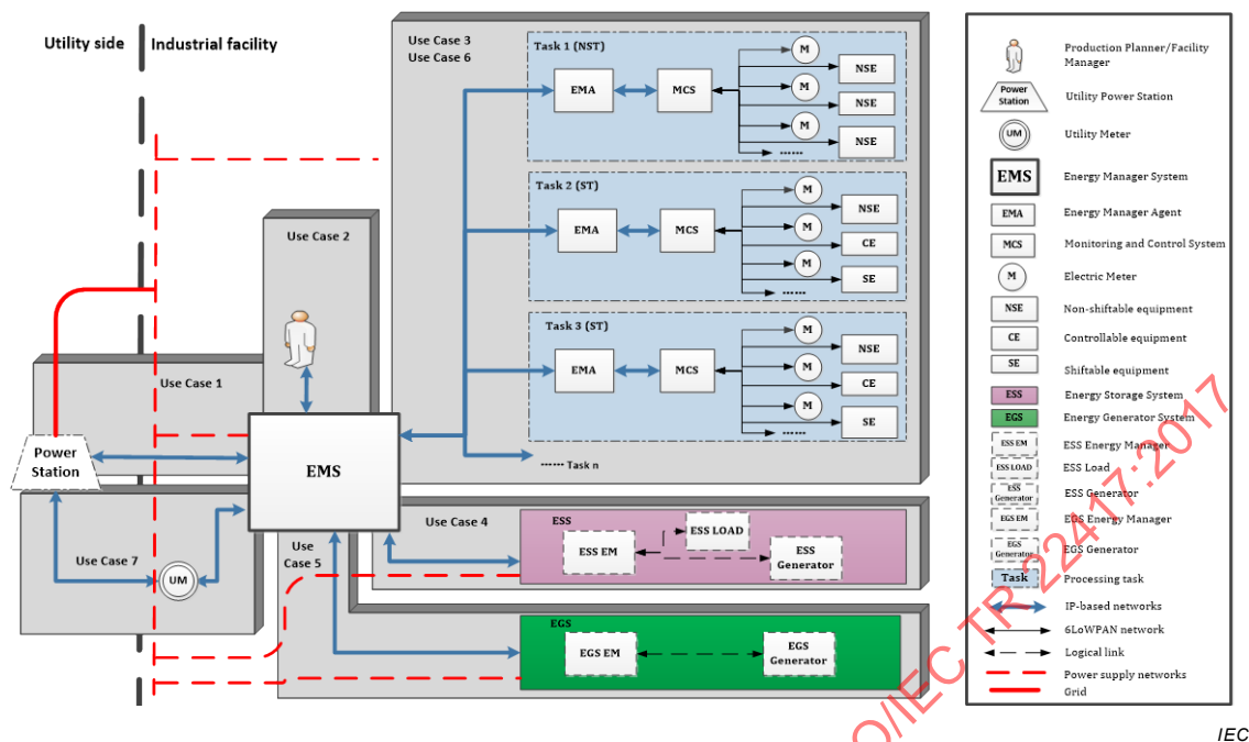
Figure 40 – Structure of IoT-Based Energy Management System with FSGIM
