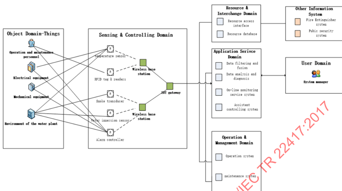
Figure 42 – System Architecture of Smart Water Plant Monitoring System
