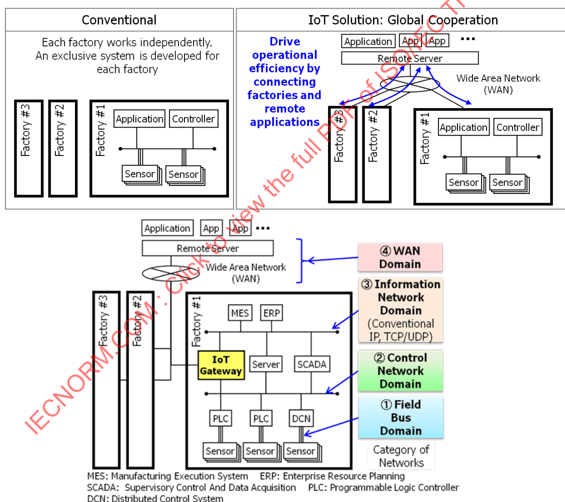
Figure 16 – Cooperation between Factories and Remote Applications
