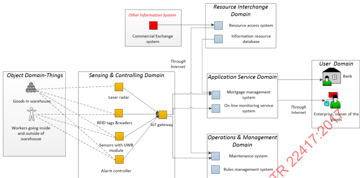
Figure 15 – Data Flow of Warehouse Goods Monitoring from architectural viewpoint
