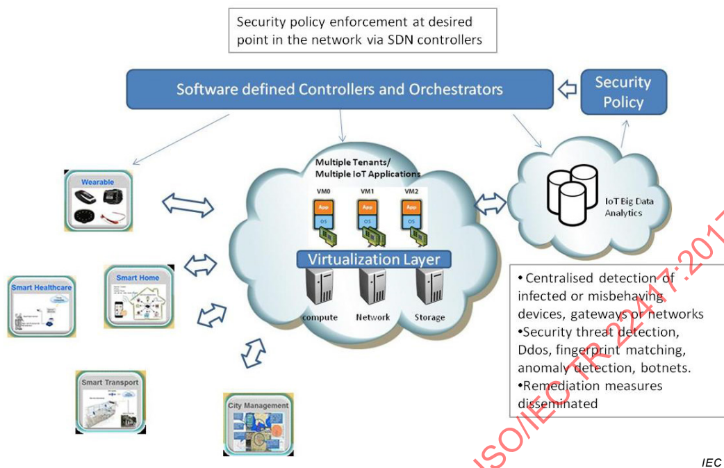
Figure 6 – IoT Security with Big Data Analytics in SDN/NFV clouds
