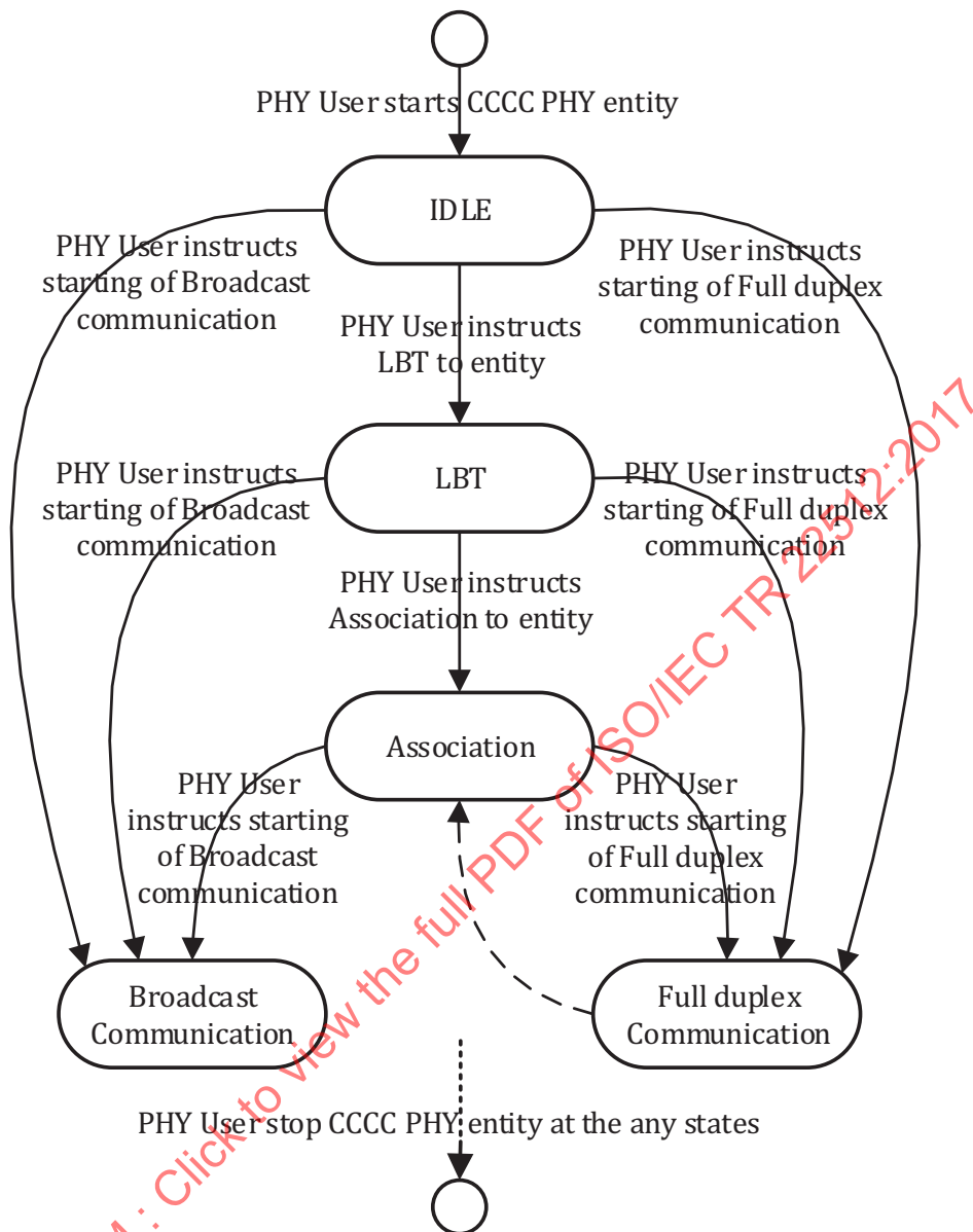
Figure 4 — Implementation as state machine
