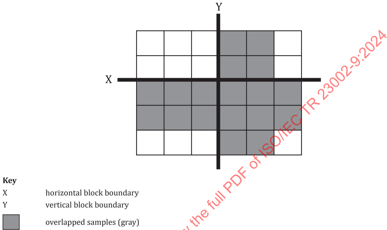
Figure 21 — Overlapped blocks
