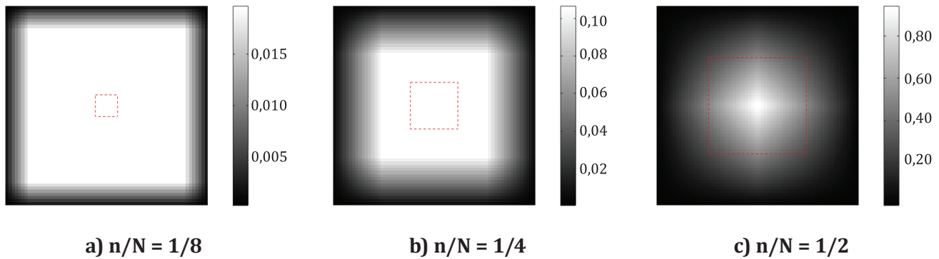
Figure 11 — Probability of (N \times N) template samples to be part of a random (n \times n) window
