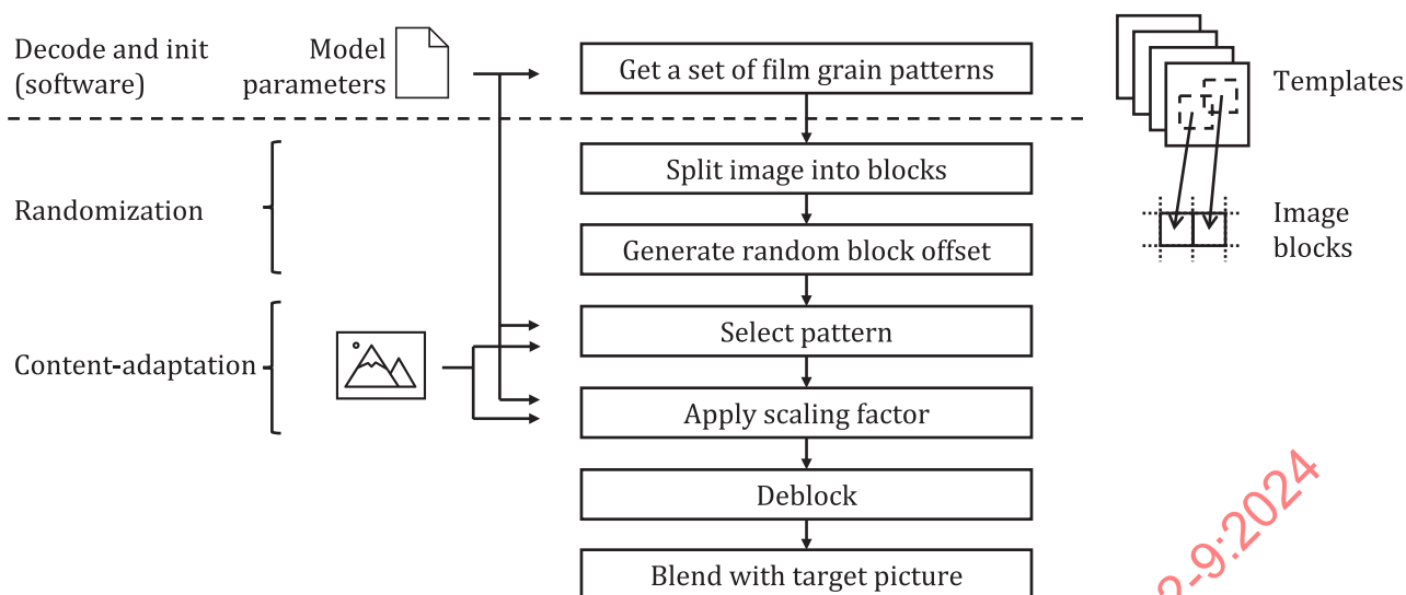
Figure 8 — Template-based film grain synthesis workflow
