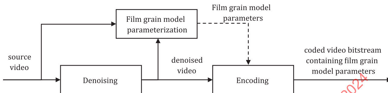
Figure 4 — Use of film grain modelling technologies with a denoising pre-processing stage
