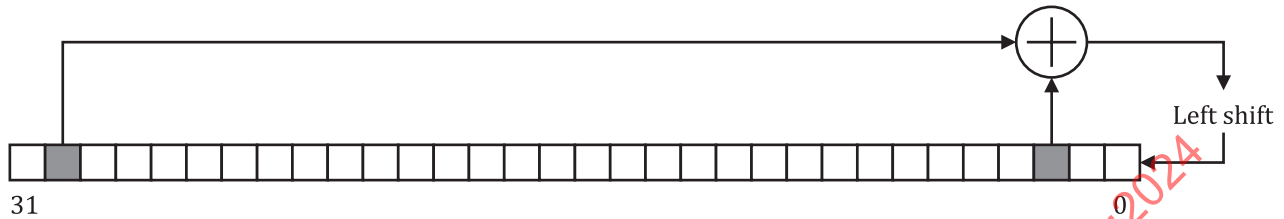
Figure 13 — LFSR with 31 st order polynomial ( x^{31} + x^3 + 1 )
