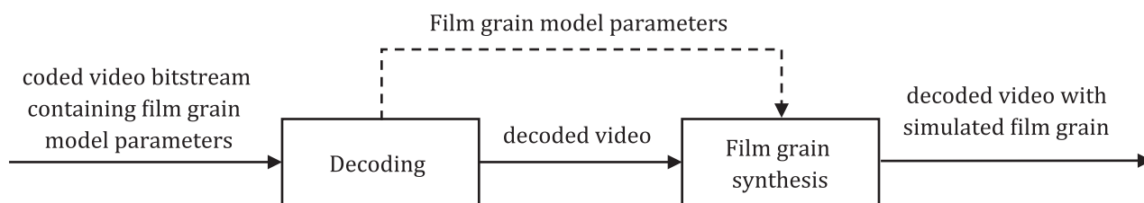
Figure 7 — Decoding process along with the film grain synthesis post-processing
