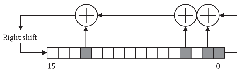
Figure 19 — LFSR used in AFGS1
