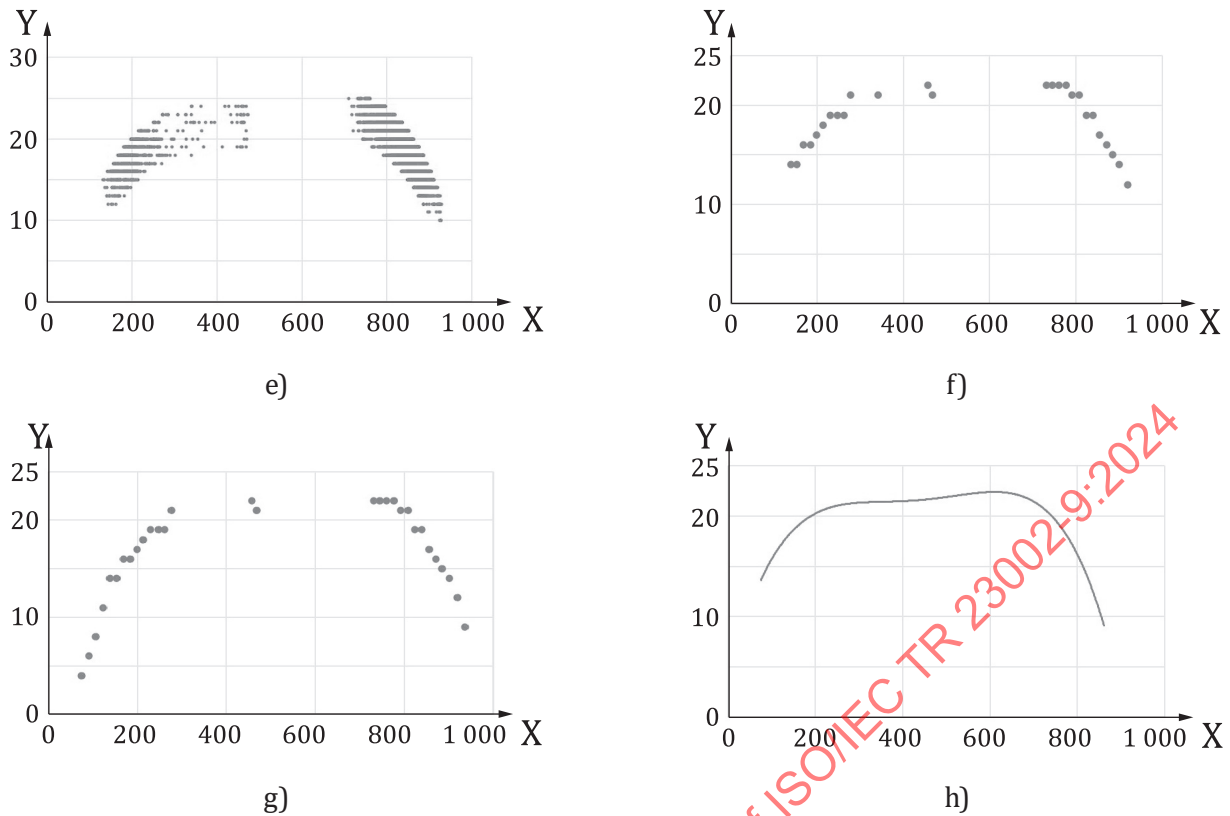
Figure 23 — Two-pass curve fitting process
