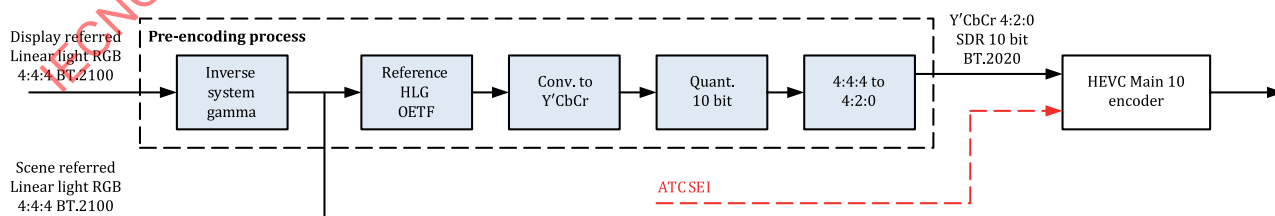
Figure 6 — Conventional HLG Y'CbCr pre-encoding process system diagram
