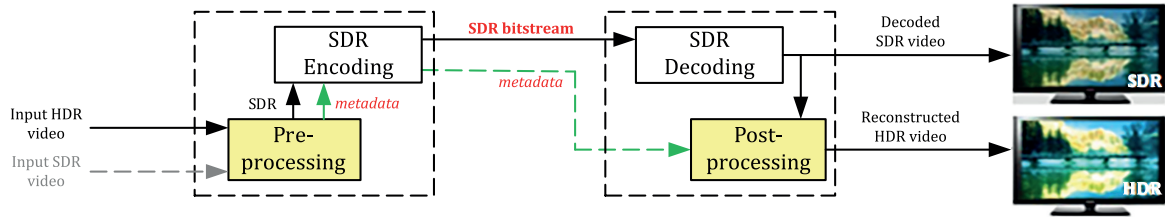
Figure 8 — Bitstream SDR backward compatibility using single layer coding system
