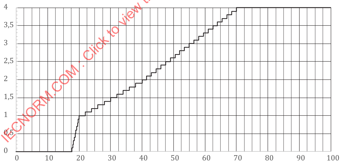
Figure 2 — Continuous grades for symbol contrast, assigned to 41 smaller grade levels
