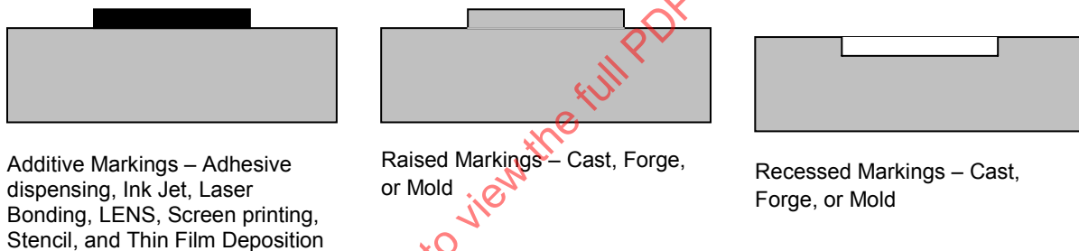
Figure B.1 — Non-intrusive marking cross sections
