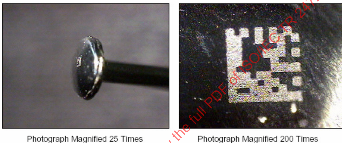
Figure A.3 — Two-dimensional symbol applied to the head of a straight pin using an excimer laser
