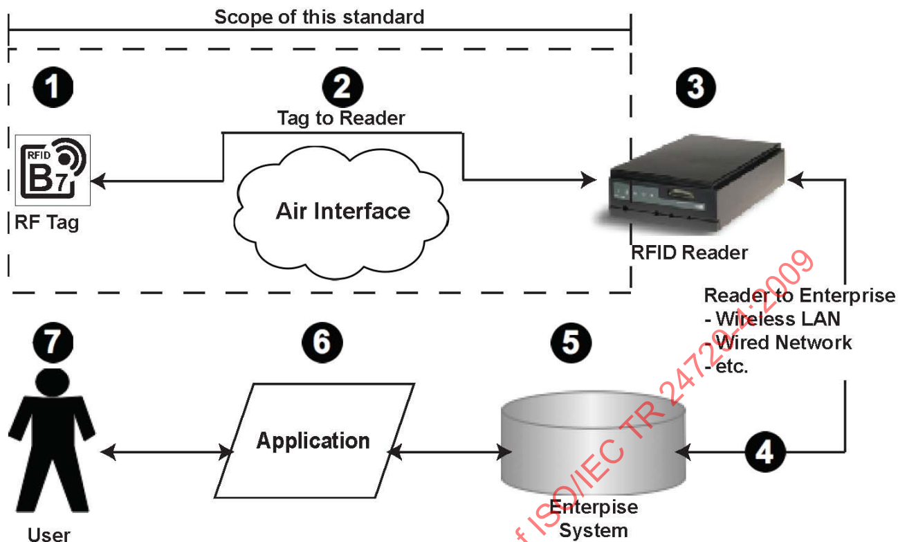
Figure 1 — RFID system top level architecture
