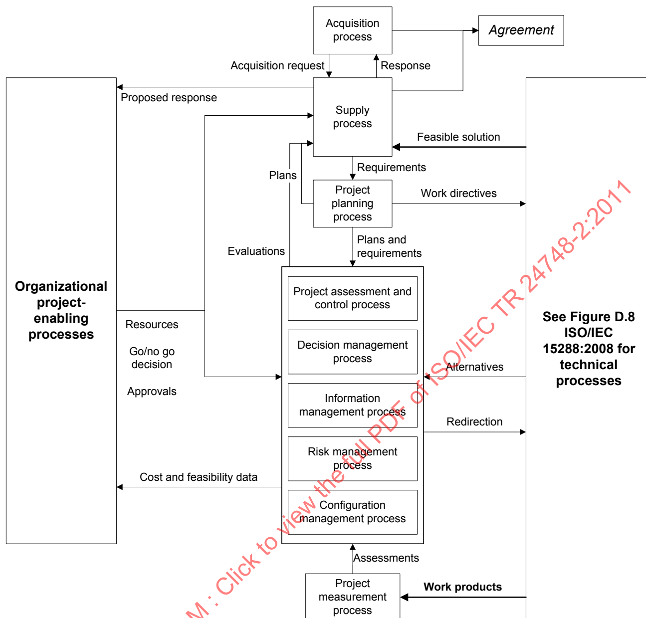
Figure 13 — Application of processes to form a formal agreement
