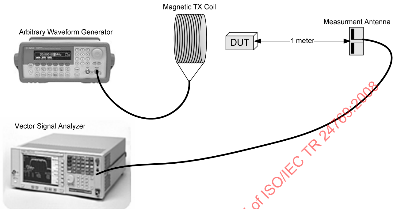
Figure 3 — Setup of equipment for optional OOK/FSK RF test
