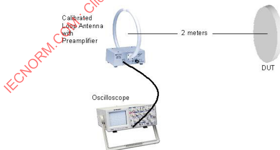
Figure 5 — Setup of equipment for exciter magnetic transmitter test
