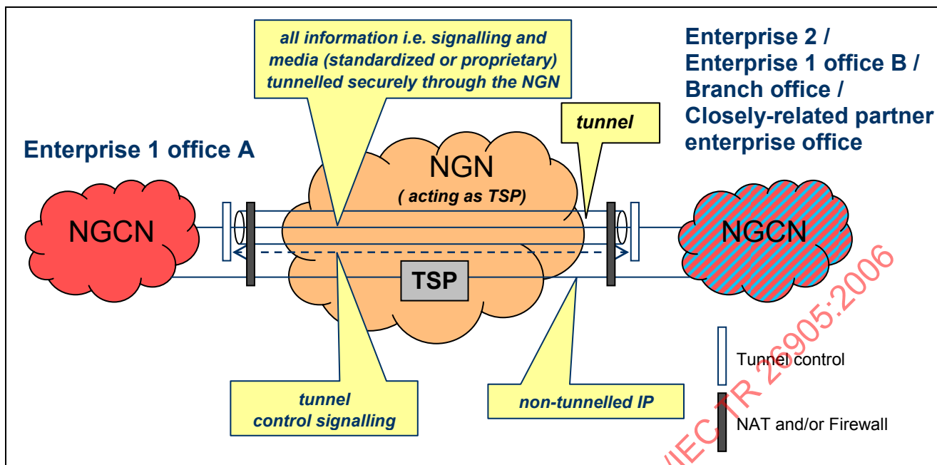
Figure 3 — Scenario 1 - Communication between NGCNs using a VPN
