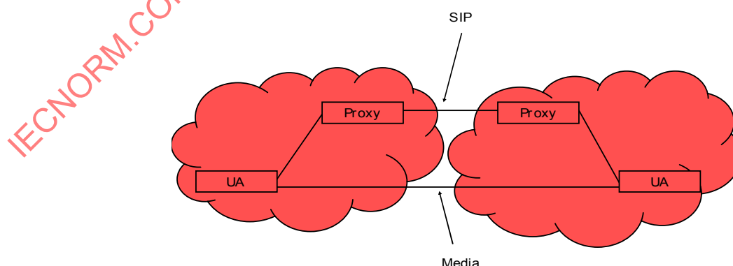
Figure 8 — Typical SIP trapezoid
