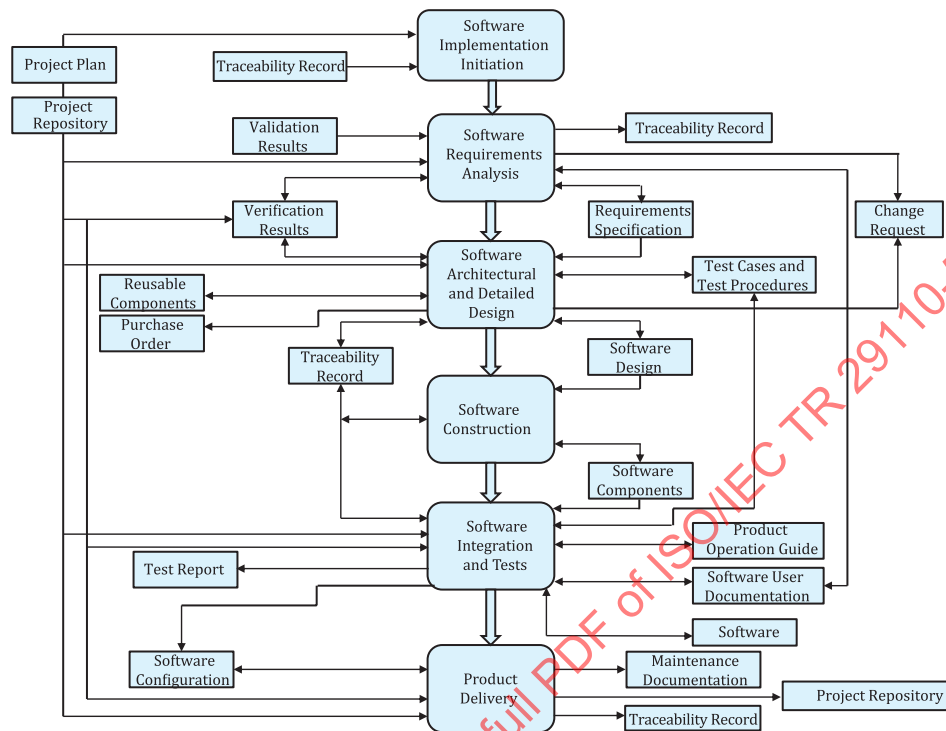
Figure 5 — Software Implementation process diagram
