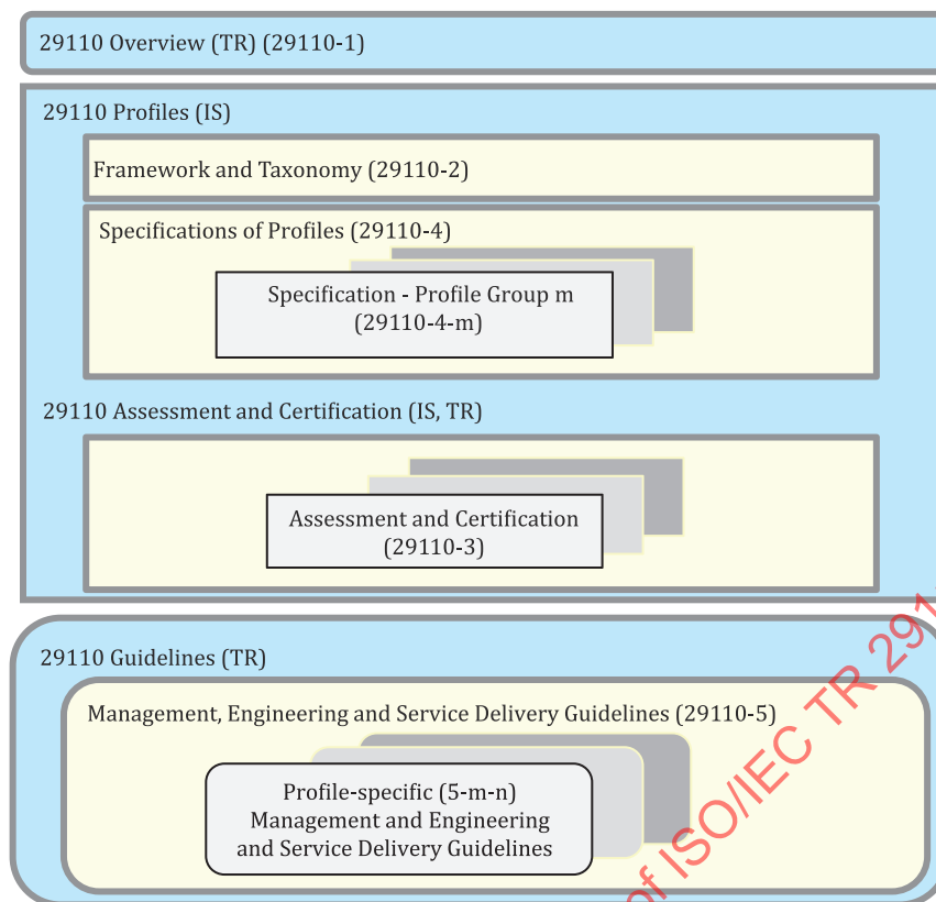
Figure 1 — ISO/IEC 29110 series
