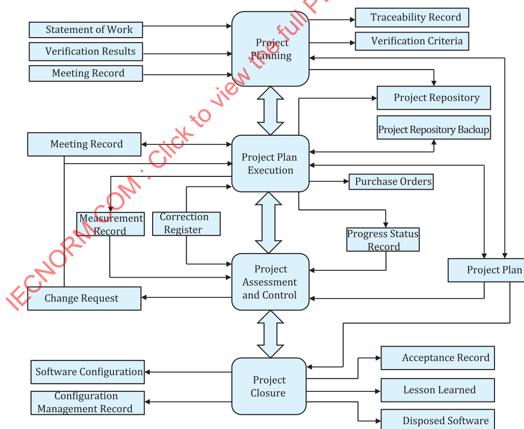
Figure 4 — Project Management process diagram
