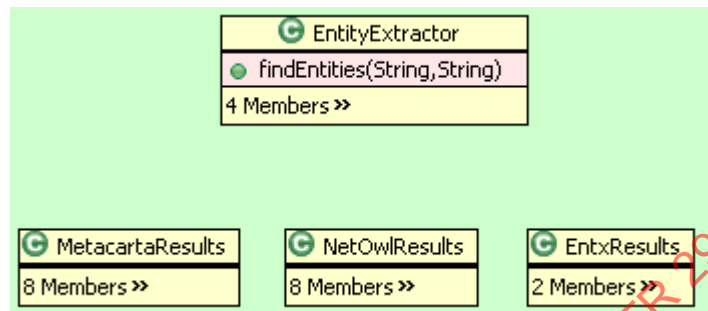
Figure 18 — EntityExtractor
