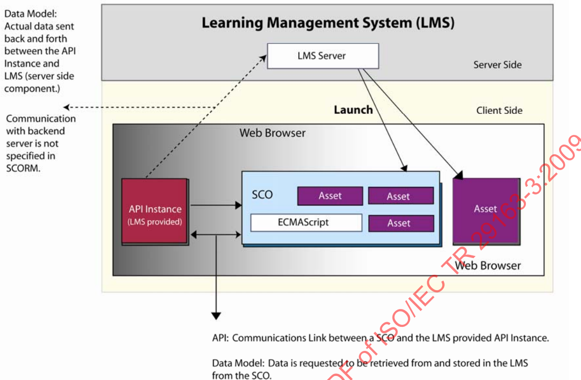
Figure 1.2a: SCORM Conceptual Run-Time Environment.
