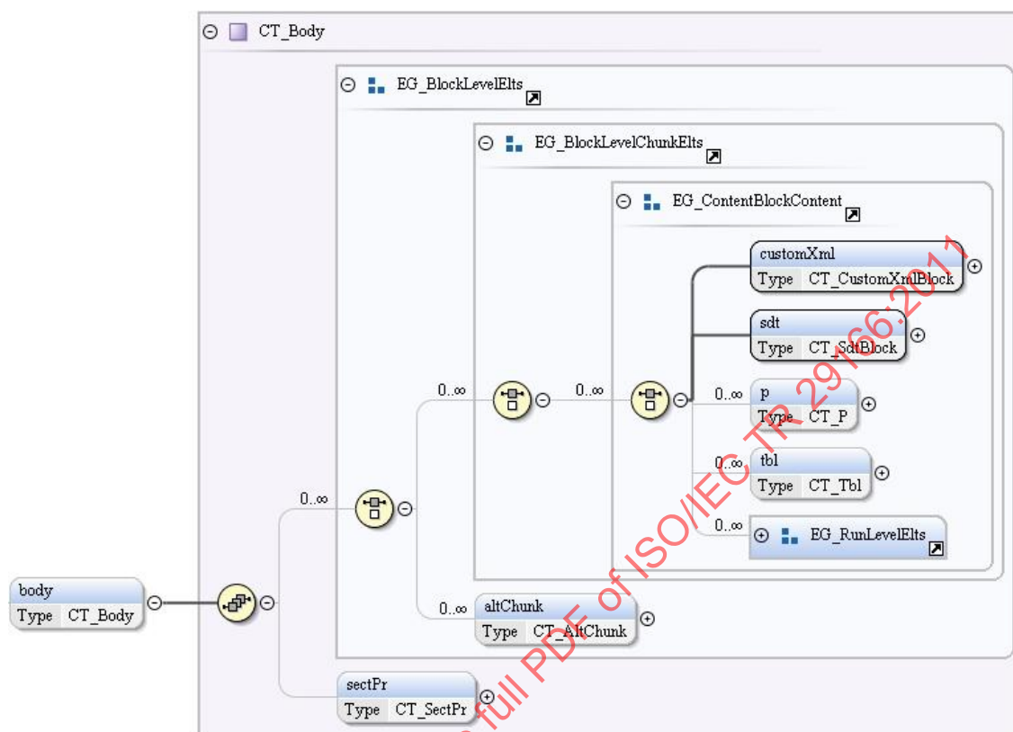
Figure 66 — XML structure of word processing documents in OOXML
