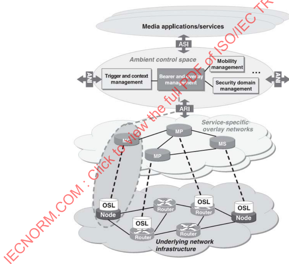
Figure B.1 — SMART Multimedia Routing and Transport Architecture
