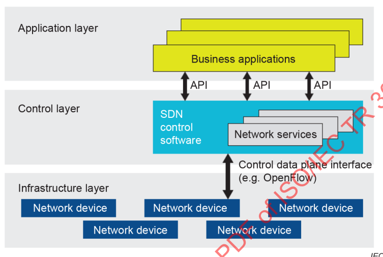
Figure 4 – Software defined network architecture
