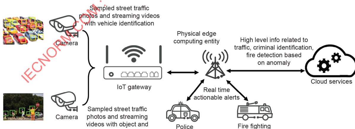
Figure 8 – Concept of video monitoring with edge computing
