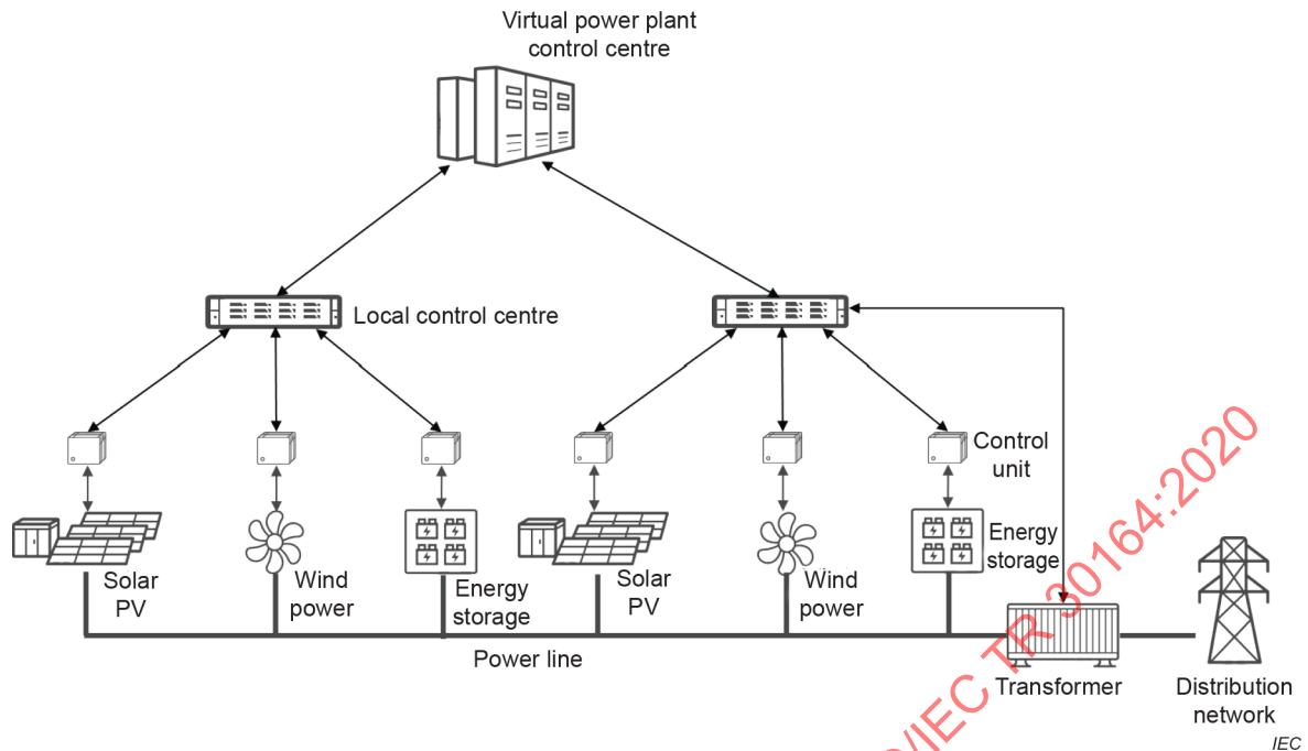
Figure 11 – Concept of centralized monitoring of power plants
