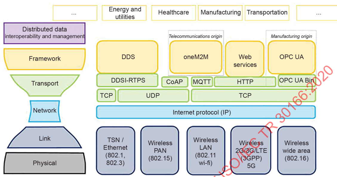
Figure 8 – IIoT connectivity stack from IICF, see [38]
