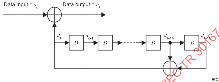
Figure 31 – Scrambler block diagram
