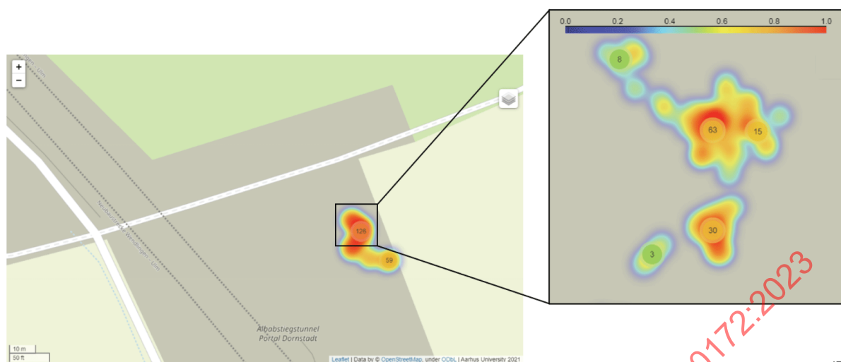
Figure B.2 – Identification of close proximity events between heavy machinery
