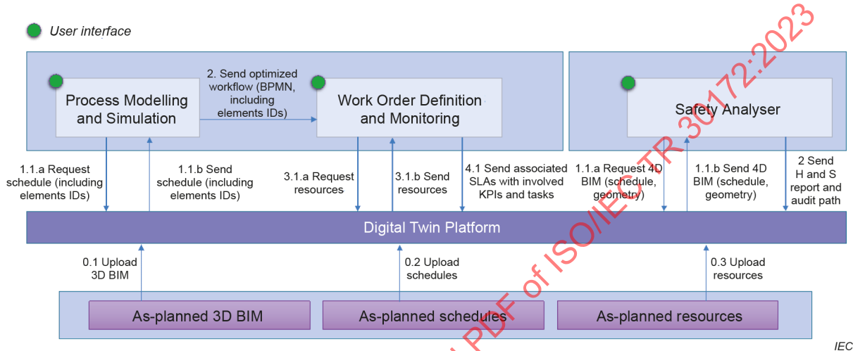
Figure B.7 – Use case diagram: before construction starts
