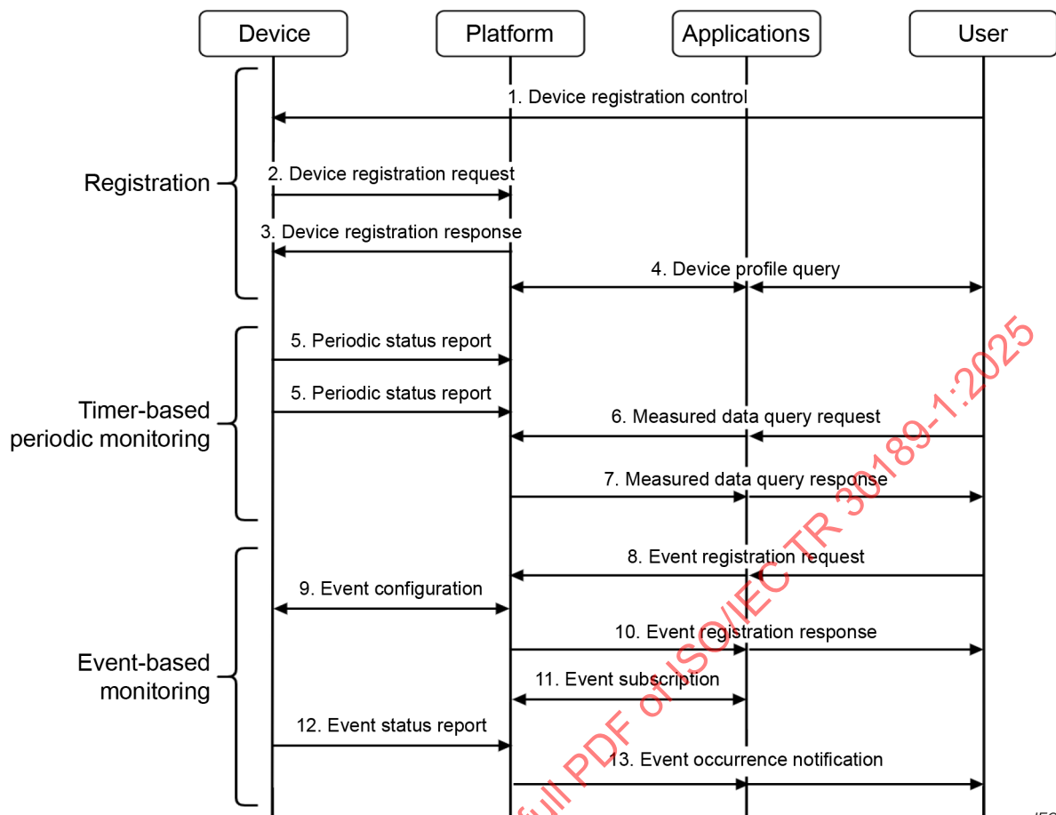
Figure 5 – Information flows for status monitoring operation
