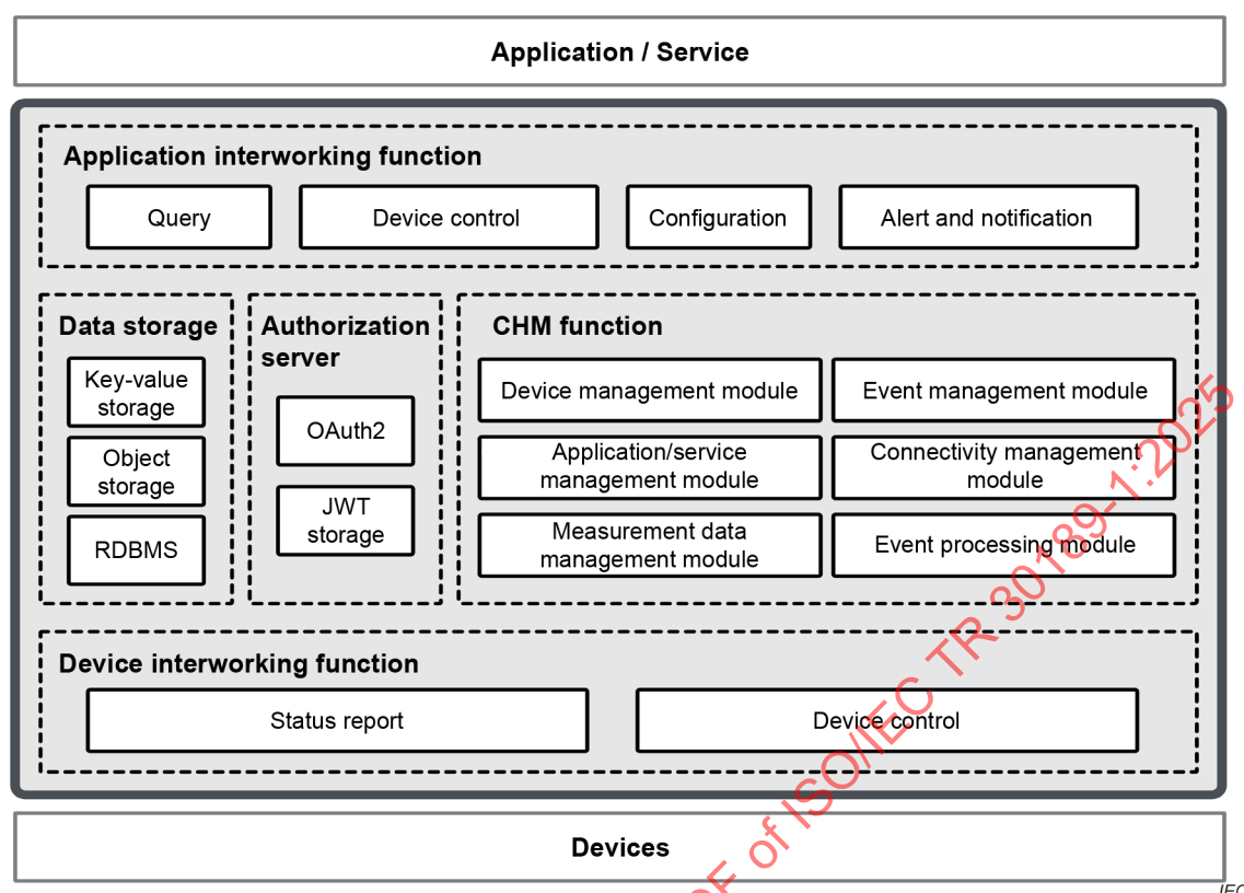
Figure 4 – Platform functions for IoT-based CHM
