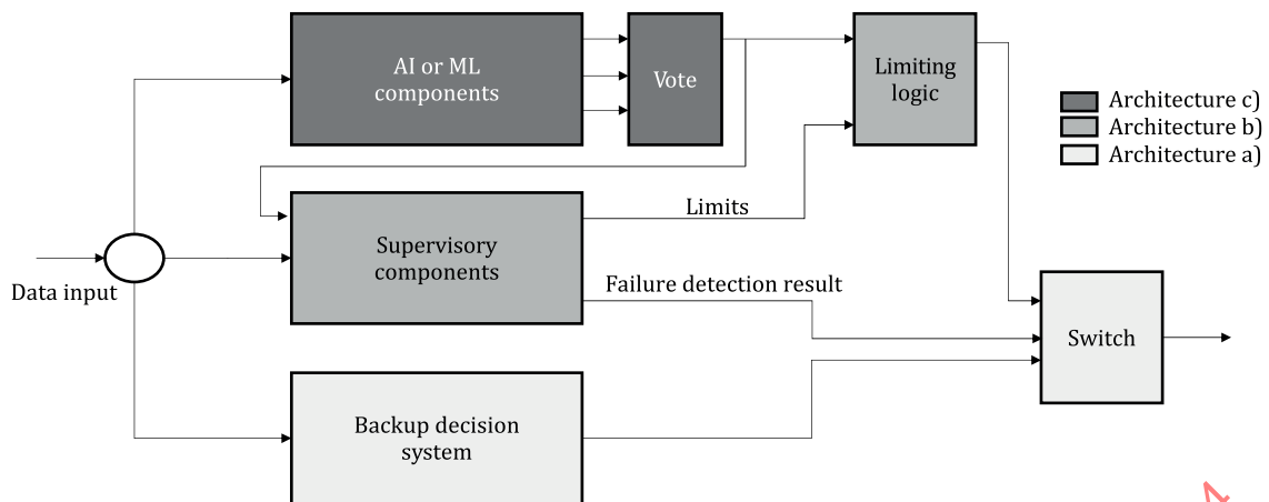
Figure 5 — Architectural patterns for systems using AI technology components
