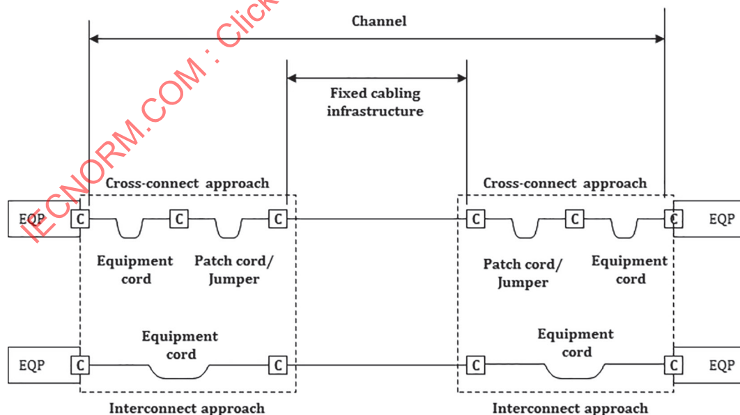
Figure 8 — Telecommunication cabling Class 1 using direct attached cords
