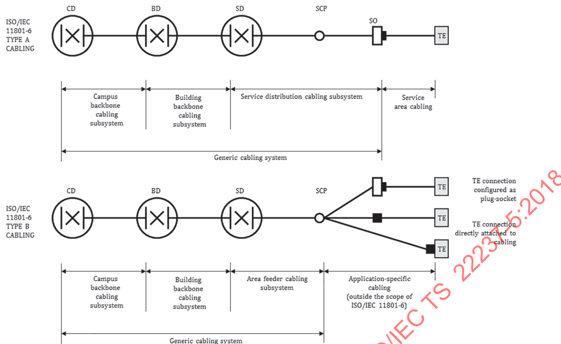
Figure 7 — Building service cabling subsystem according to ISO/IEC 11801-6
