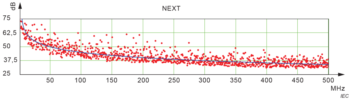
Figure 5 – Graphical example of a NEXT calculation showing statistical results (red) and final calculation (blue)
