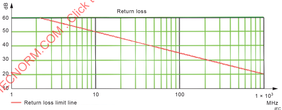
Figure 7 – 100 m cable return loss without reflection at both ends
