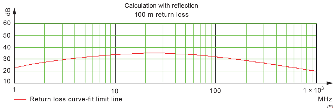
Figure 8 – 100 m cable return loss with a reflection of 0,03 at both ends (6 \Omega mismatch, ~23 dB return loss at 1 MHz)
