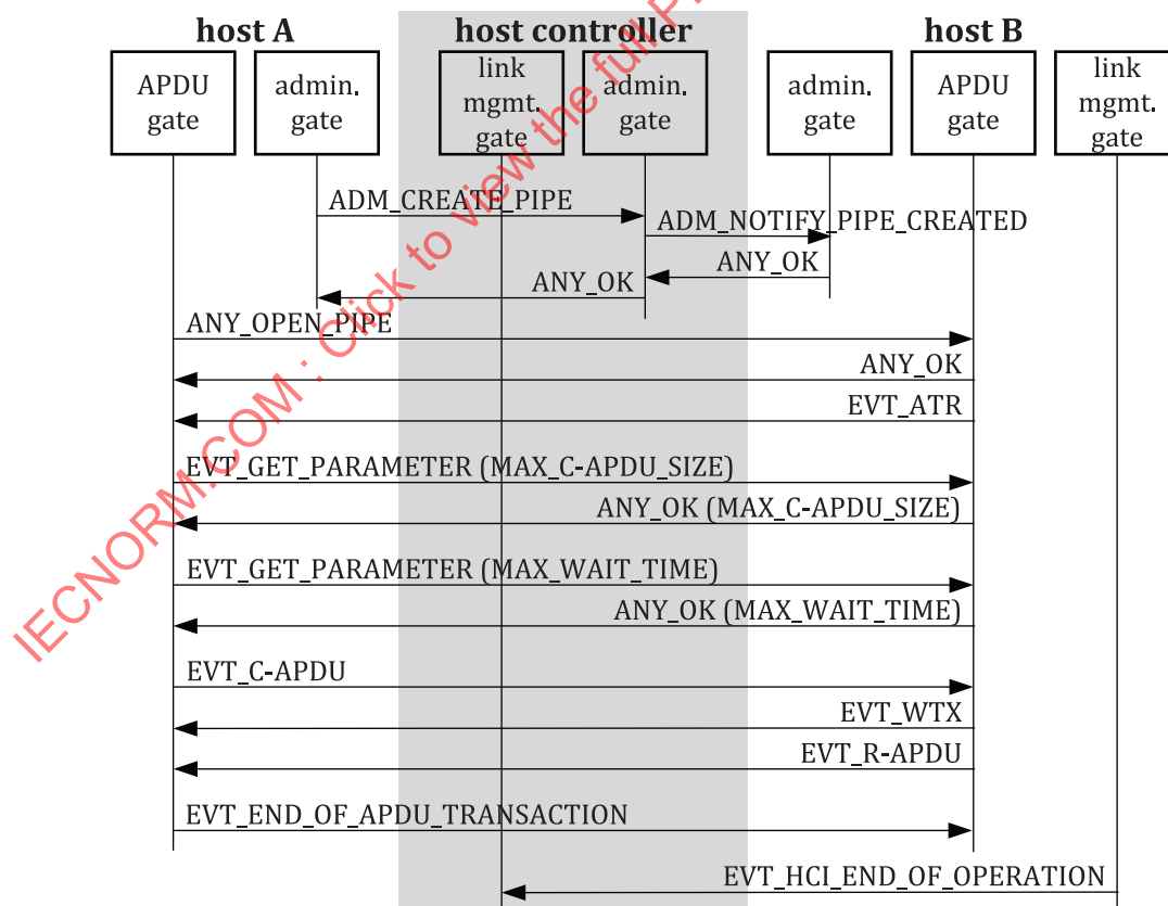
Figure 4 — Use of client and server APDU gates
