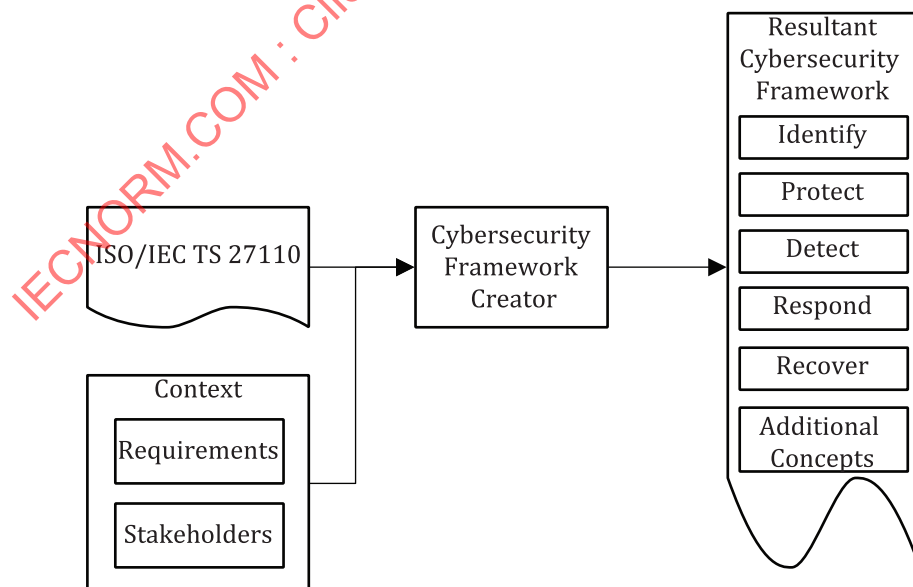
Figure 1 — Creating a cybersecurity framework using ISO/IEC TS 27110
