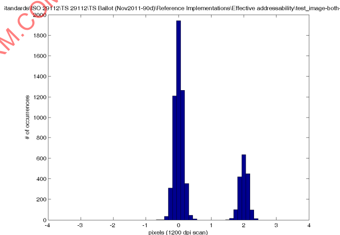
Figure D1. Expected results for effective addressability
