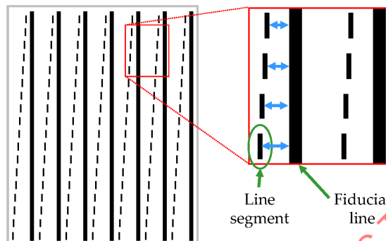
Figure 2. Effective Addressability test chart.
