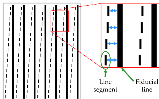
Figure A2. Effective Addressability test chart.
