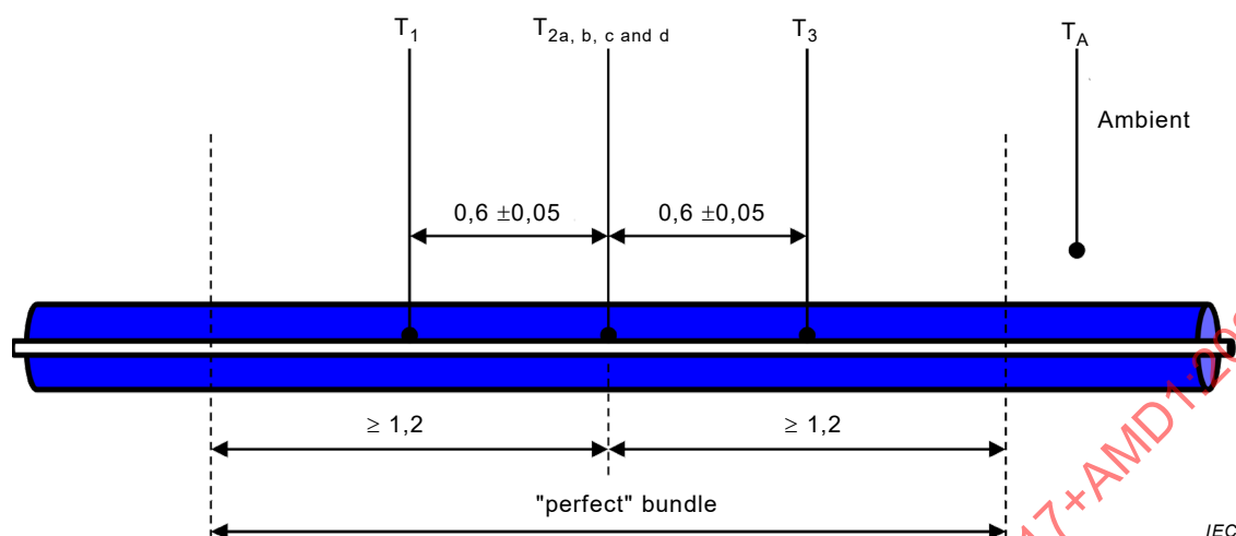
Figure E.2 – "Perfect bundle" and thermocouple configuration
